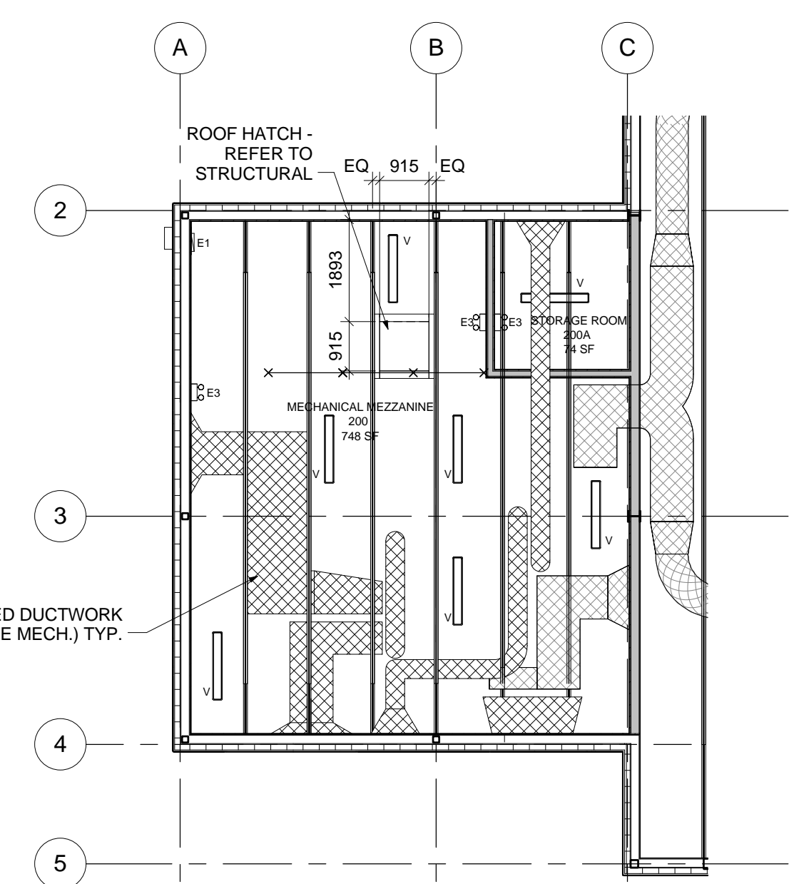
2 MEZZANINE RCP 1:100
