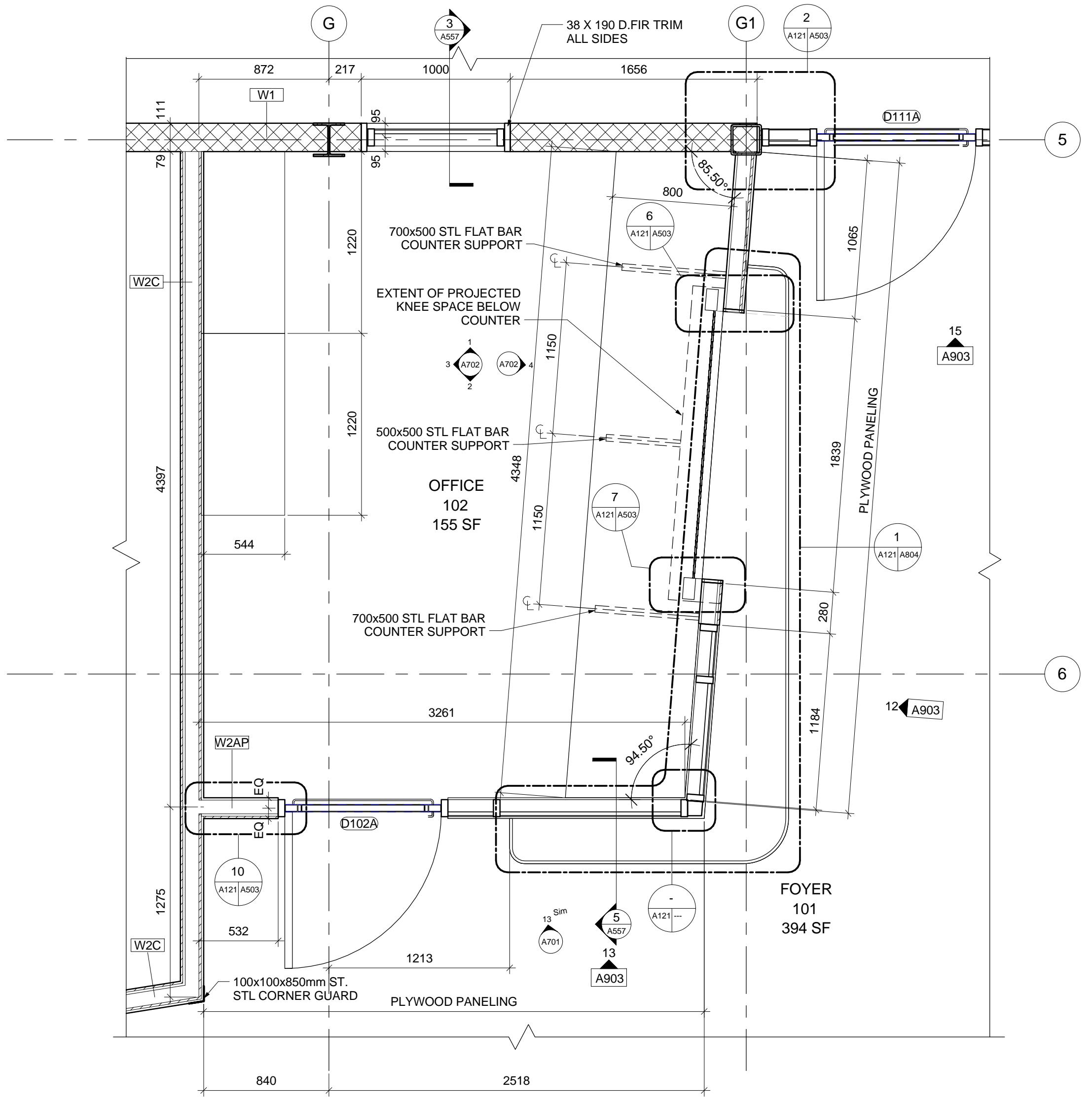
2 LARGE SCALE PLAN - RM 102 1:25
