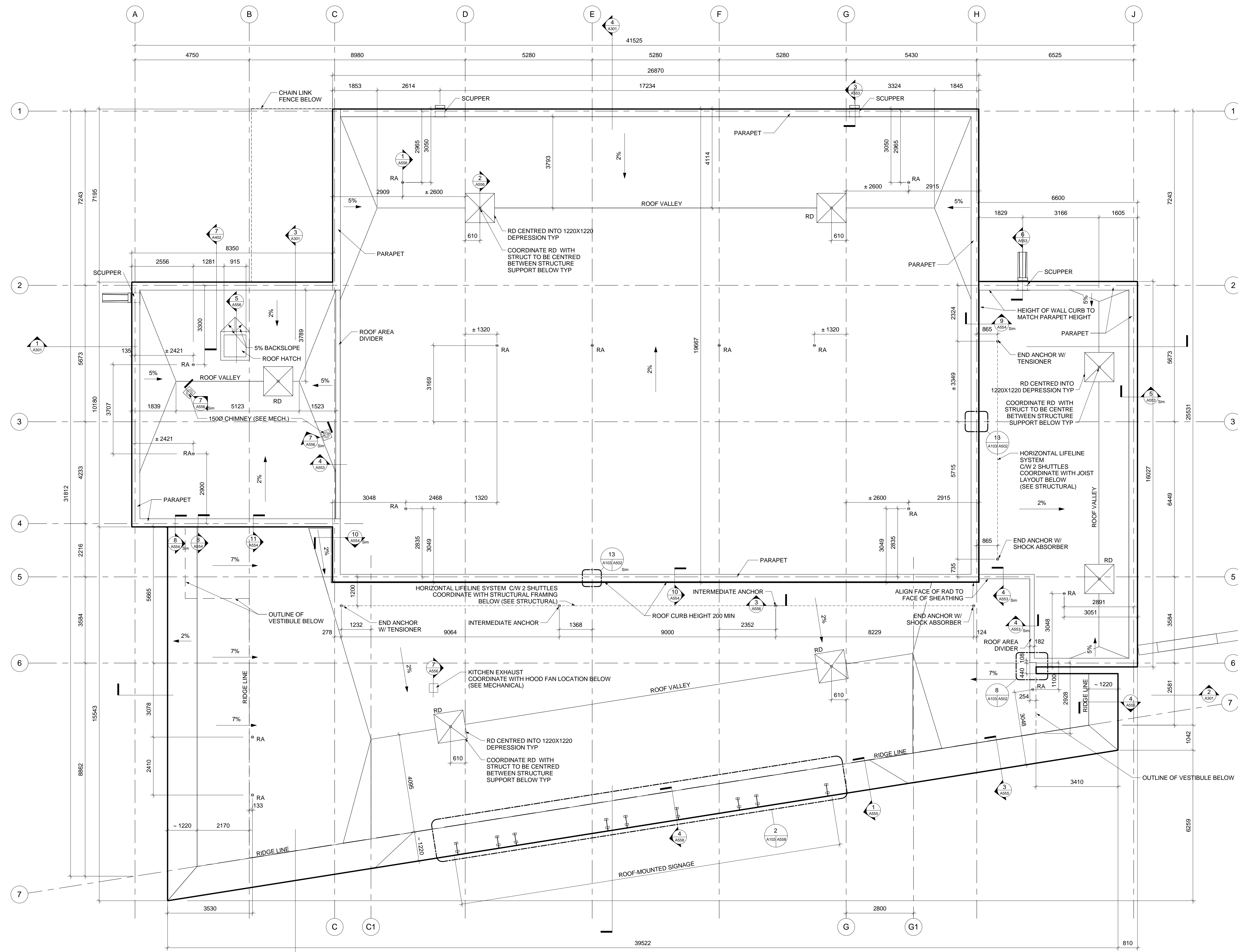
1 ROOF PLAN 1:75
