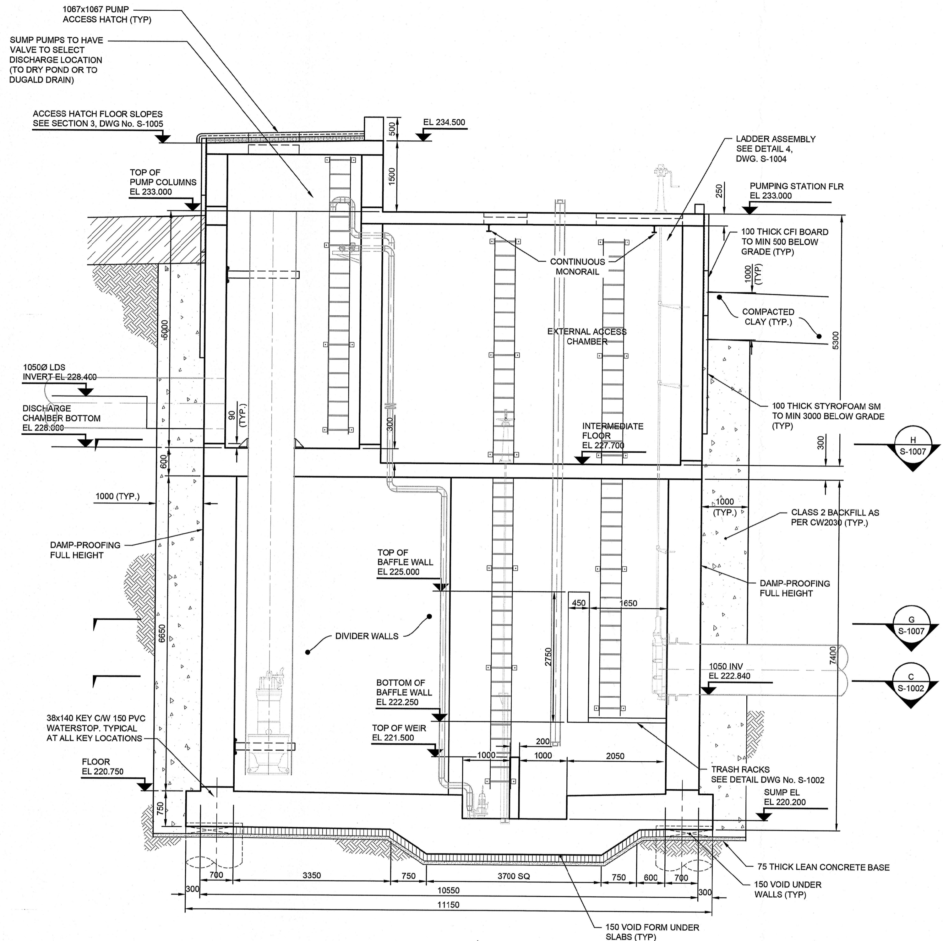
A SECTION S-1001 0 1250 2500 1:50
