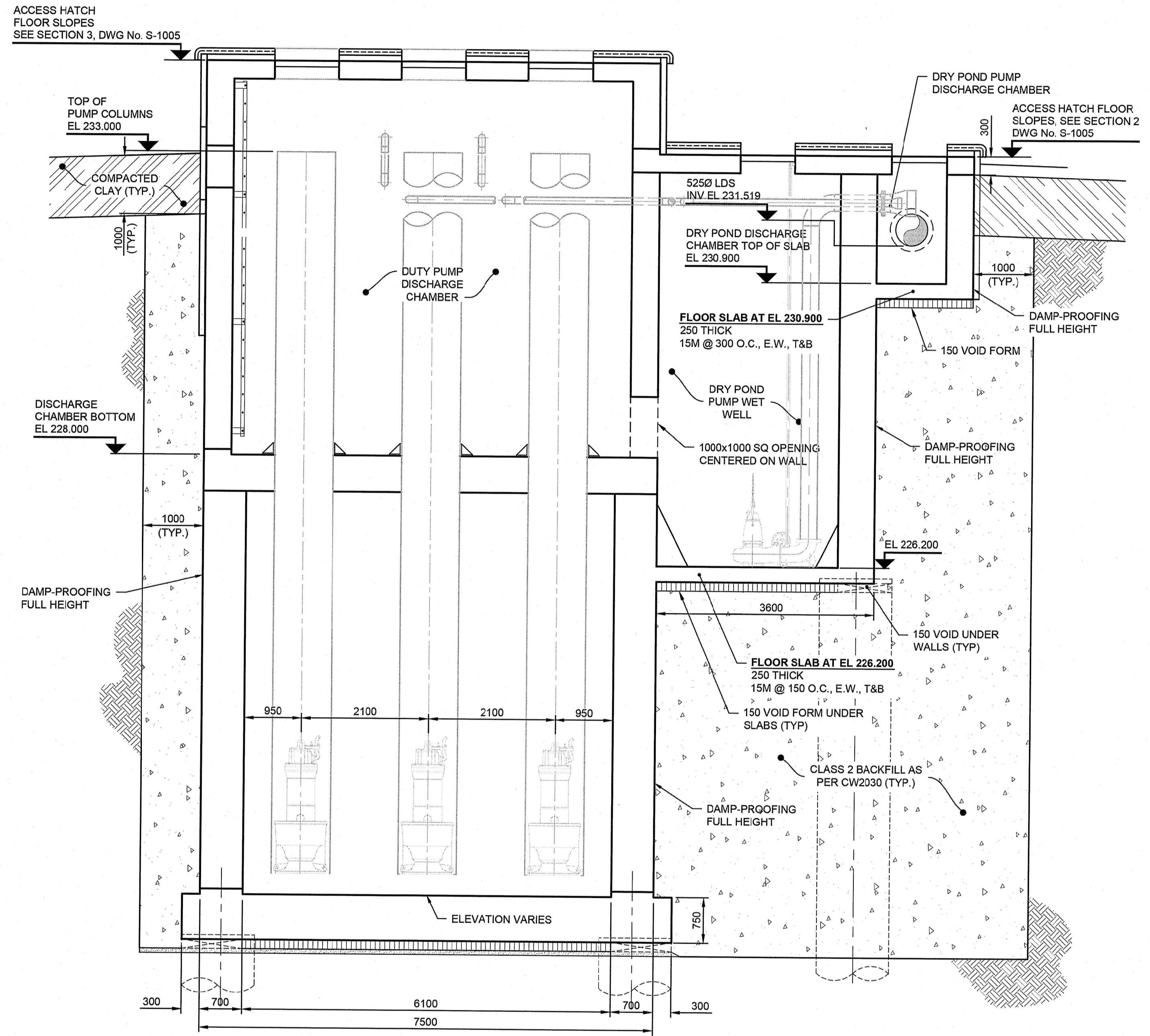
B SECTION S-1001 0 1250 2500 1:50
