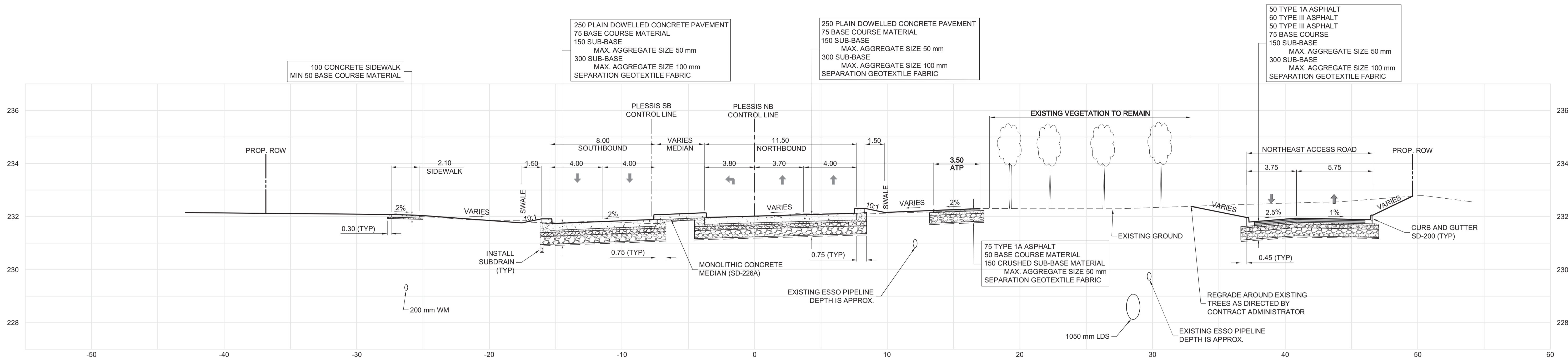
H | PLEISSIS ROAD - STA. 2+440 (NORTHBOUND) CT-0032 CT-0045 Scale: H-150 V-1:75
