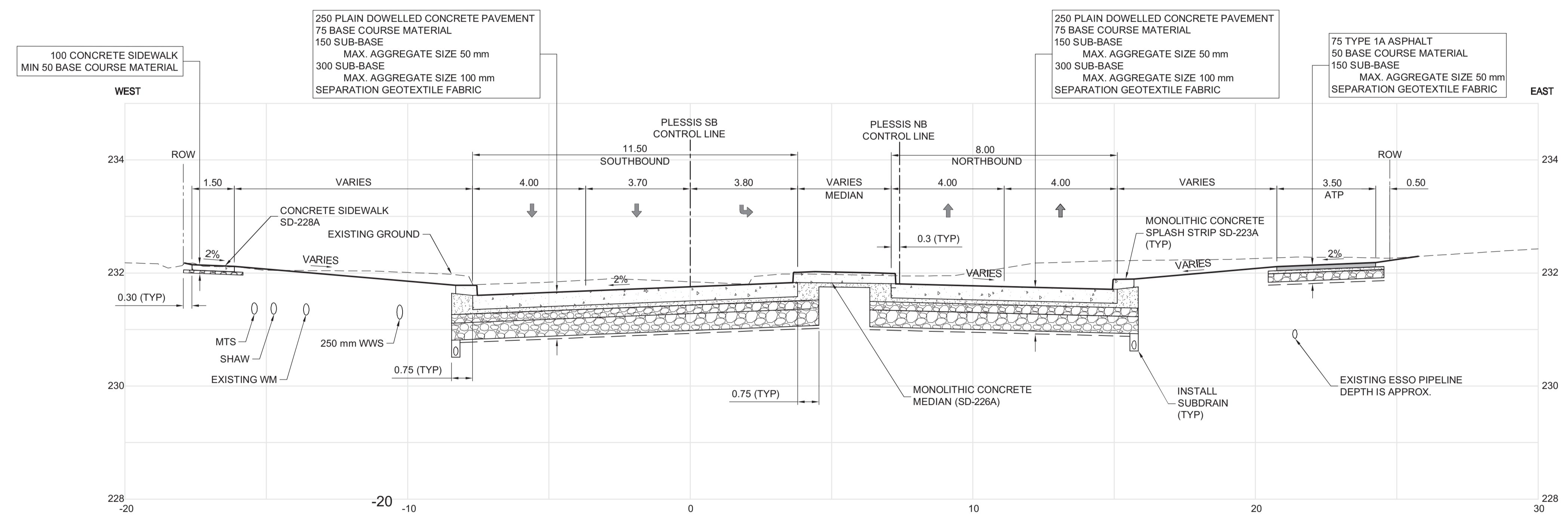
I | PLEISSIS ROAD - STA. 2+490 (SOUTHBOUND) CT-0035 Scale: H-100 V-1:50
