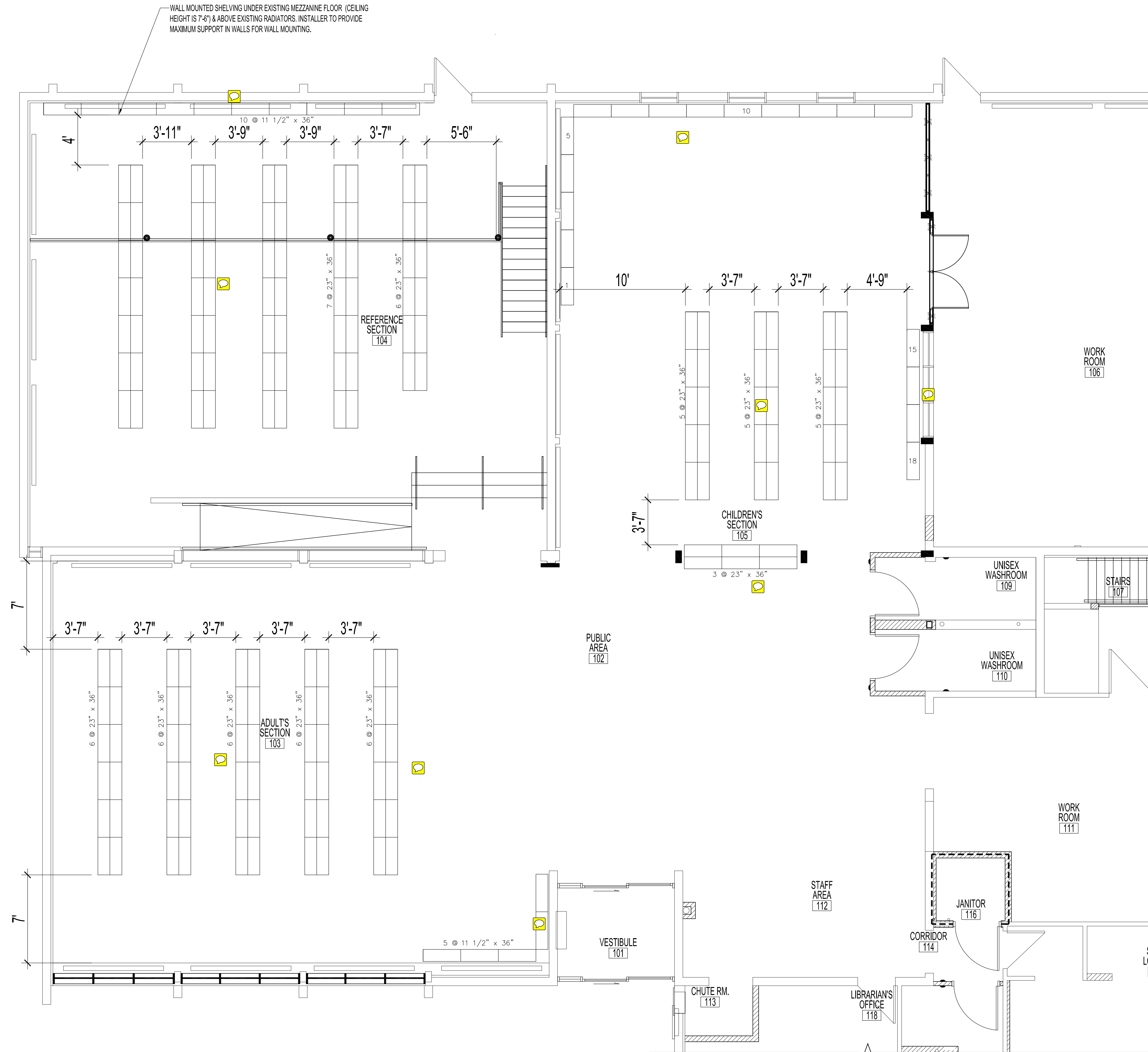
1 MAIN FLOOR PLAN - BOOK SHELVING PLAN SCALE: 1/4"=1'-0"
