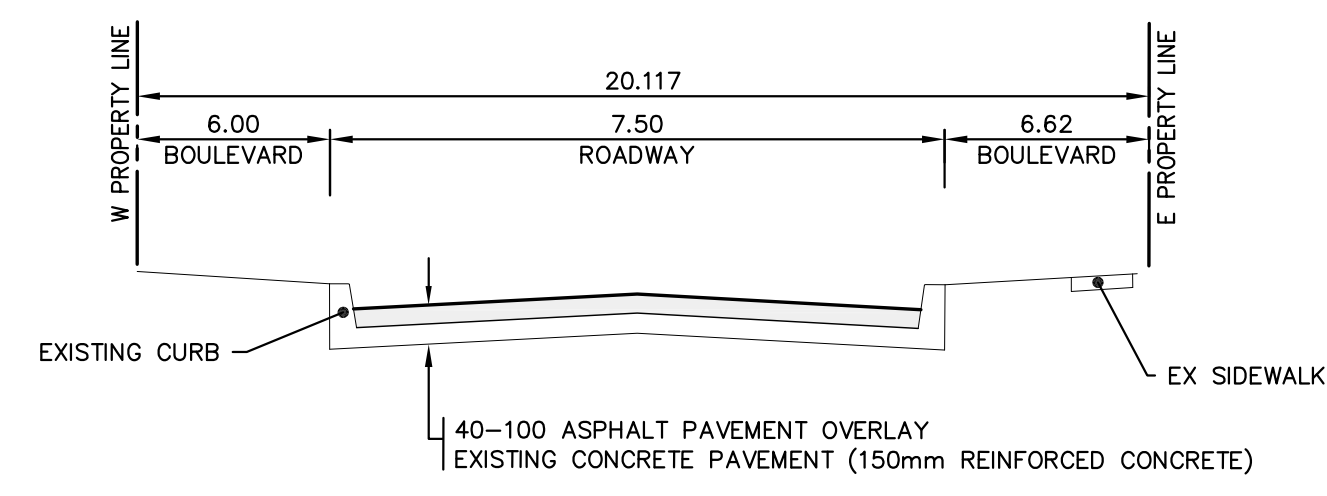
TYPICAL CROSS-SECTION NTS
