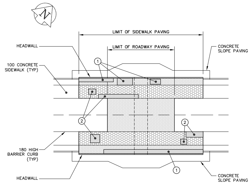
C-369 ISLAND LAKES DRIVE CULVERT N.T.S.
