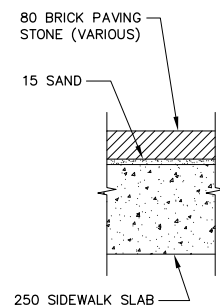
PAVING DETAIL (TYP) N.T.S.
