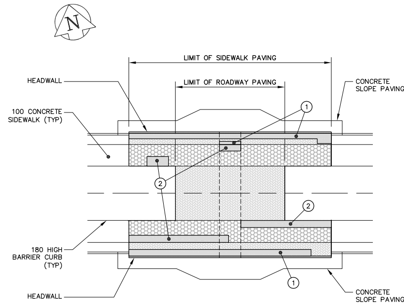
C-374 ISLAND LAKES DRIVE EAST CULVERT N.T.S.
