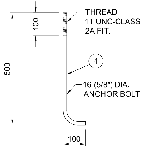
ANCHOR BOLT FOR TYPE L TRAFFIC SIGNAL BASE NTS
