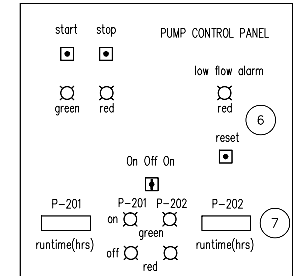
2 PUMP CONTROL PANEL SCALE: NTS
