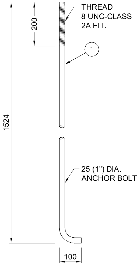
ANCHOR BOLT FOR TYPE A TRAFFIC SIGNAL BASE NTS
