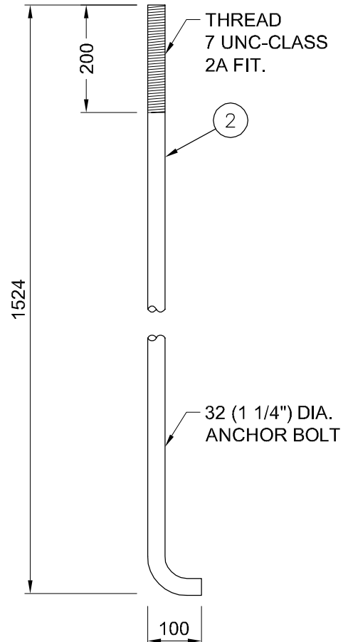
ANCHOR BOLT FOR TYPE G & D TRAFFIC SIGNAL BASE NTS
