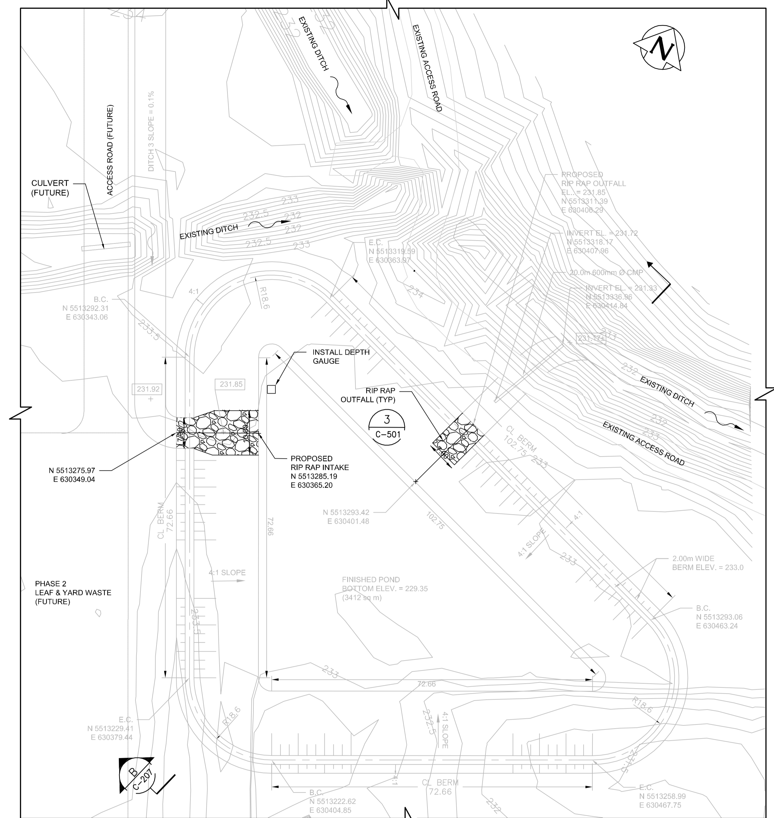
2 LEAF & YARD WASTE POND PLAN (BY OTHERS) 1:500
