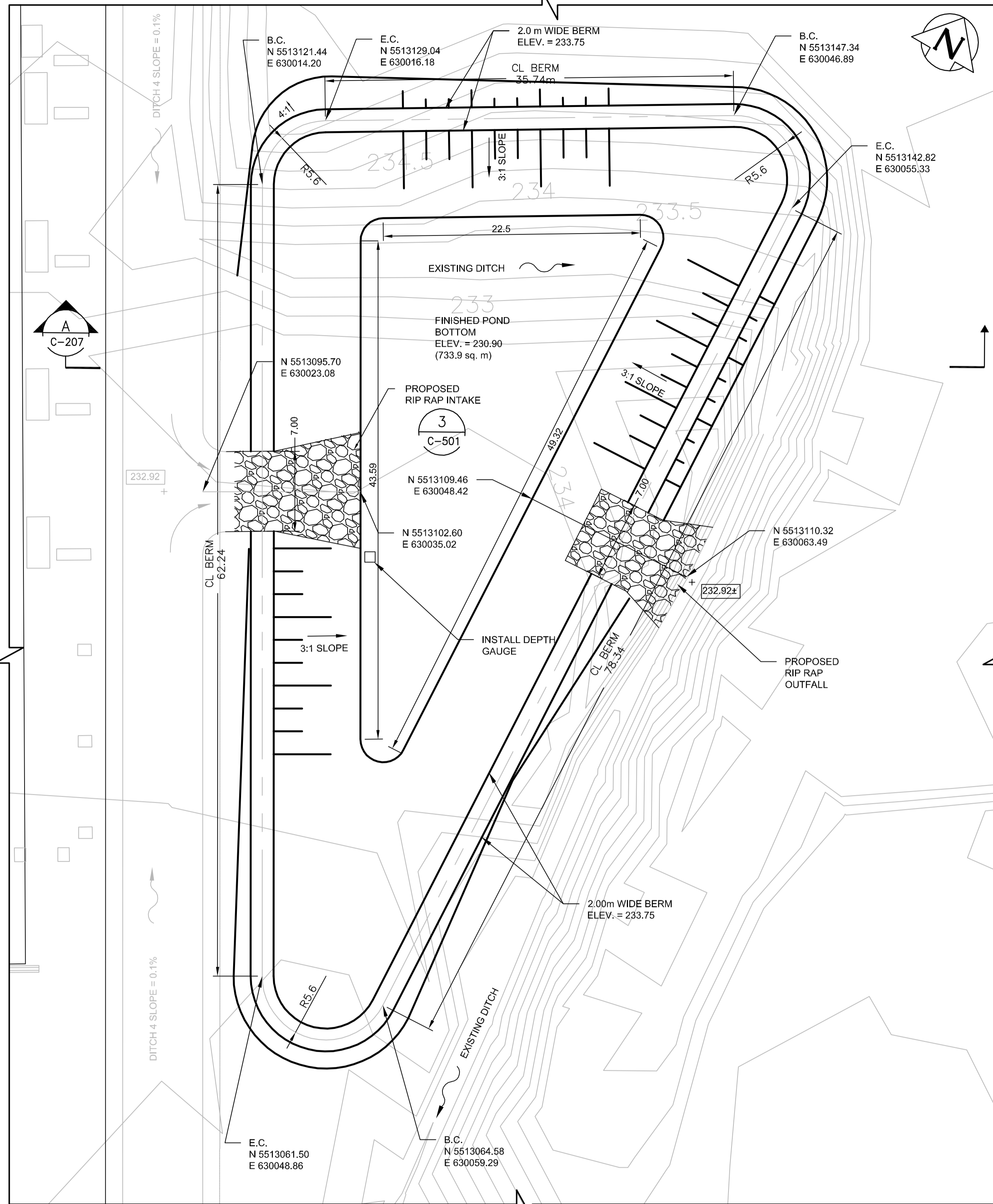
1 BIOSOLIDS POND PLAN 1:250
