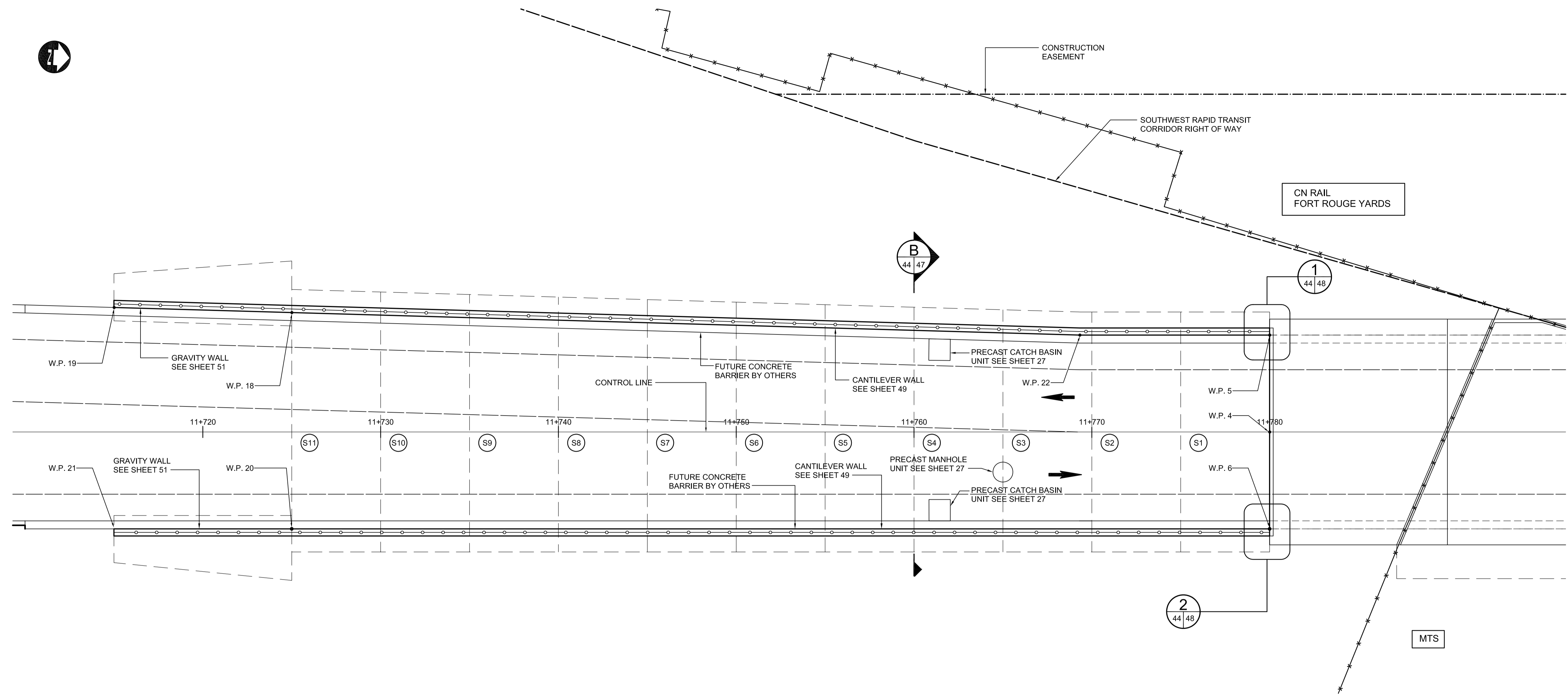
SOUTH RETAINING WALL LAYOUT SCALE 1:125
