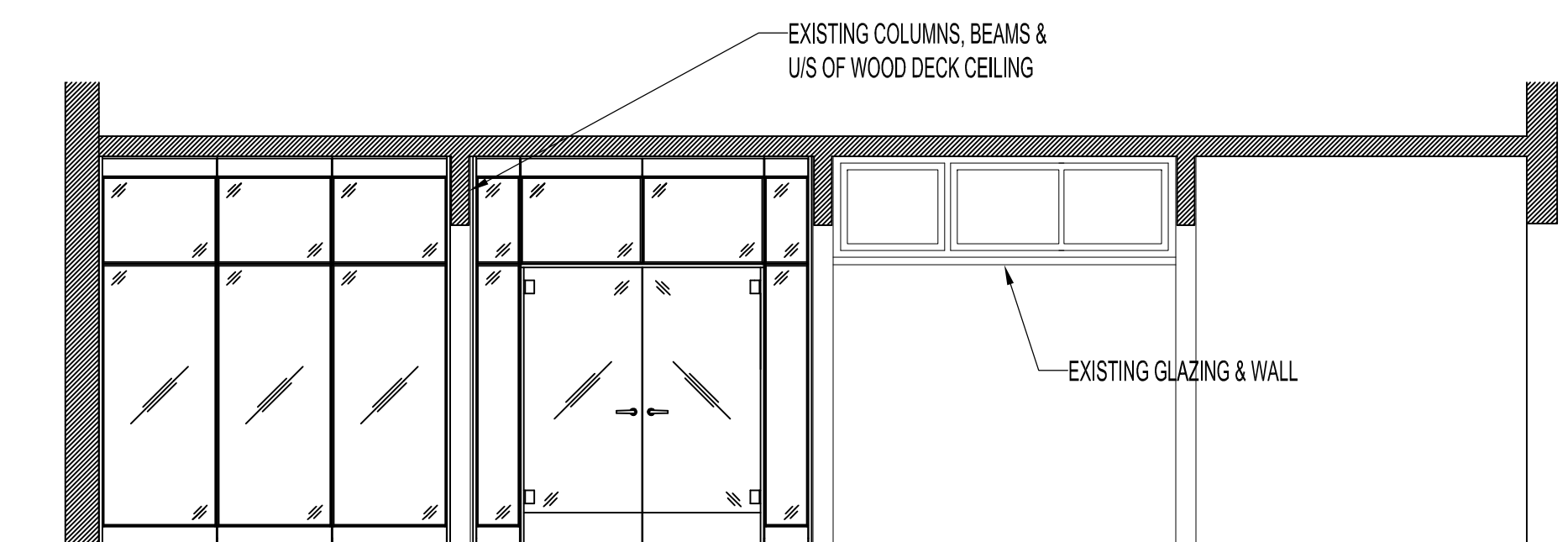
ELEVATION C1 - PANELS & DOOR IN LOCATION SCALE: 1/4"=1'-0"
