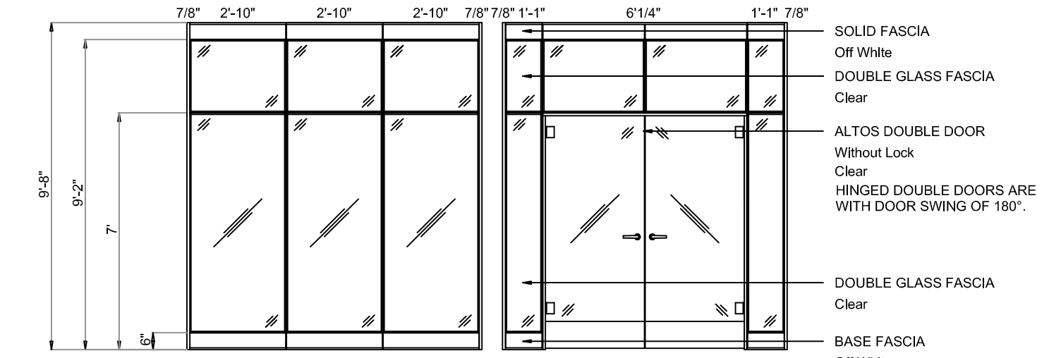
ELEVATION C2 - PANELS & DOOR DIMENSIONS & COMPONENTS SCALE: 1/4"=1'-0"
