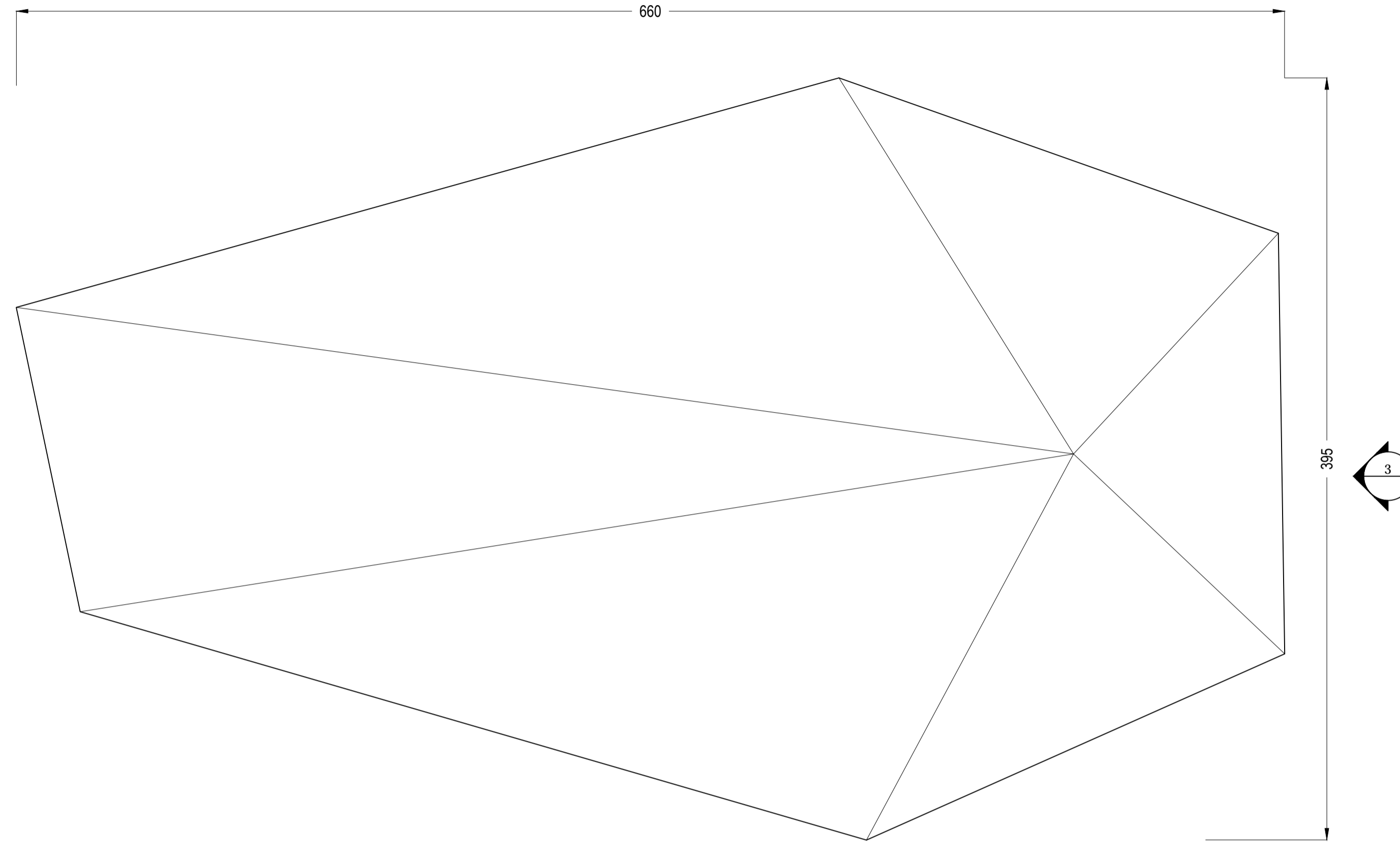
2 PR-03 REAR REFLECTOR PLAN VIEW 1:2 @ A1
