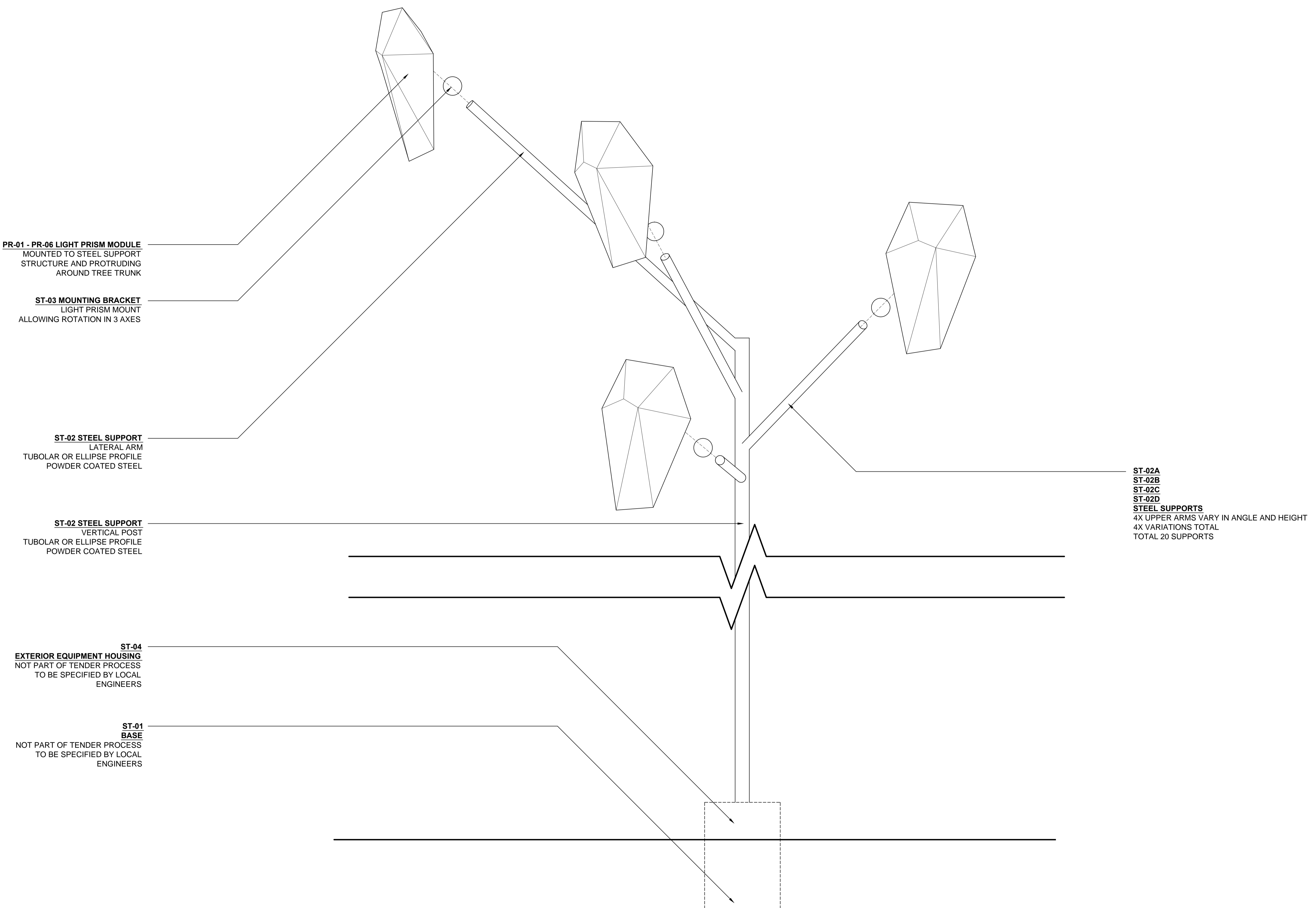
1 GENERAL ASSEMBLY ELEVATION Scale: 1:10 @ A1
