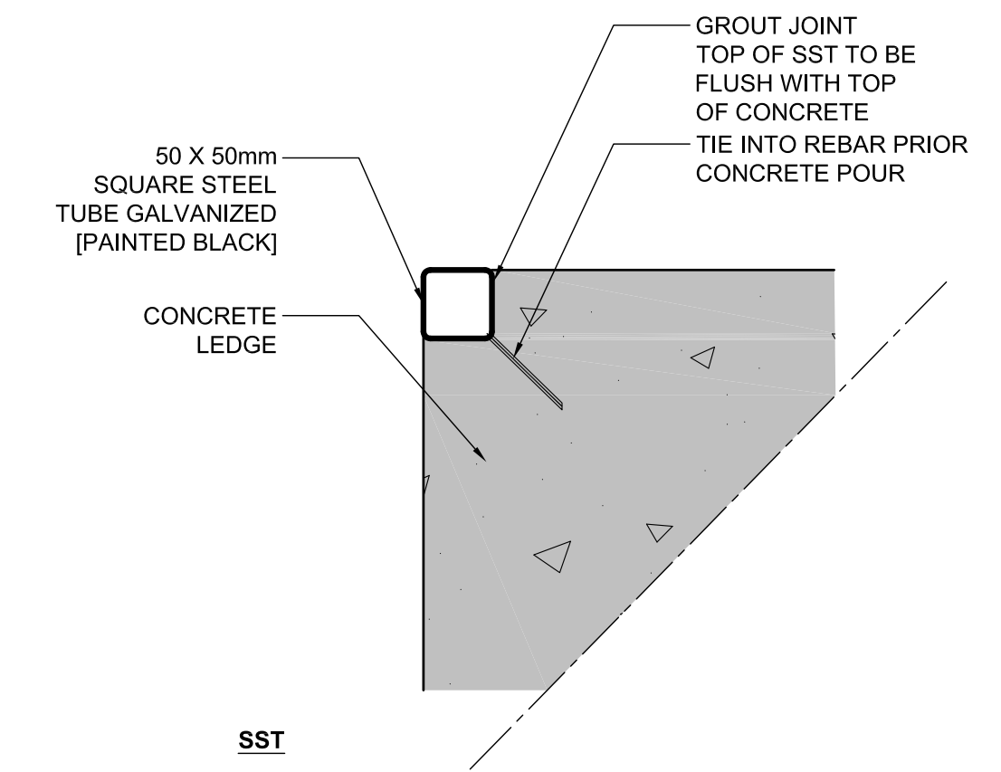
2 SQUARE STEEL TUBE PLACEMENT L9 SCALE - 1 : 5
