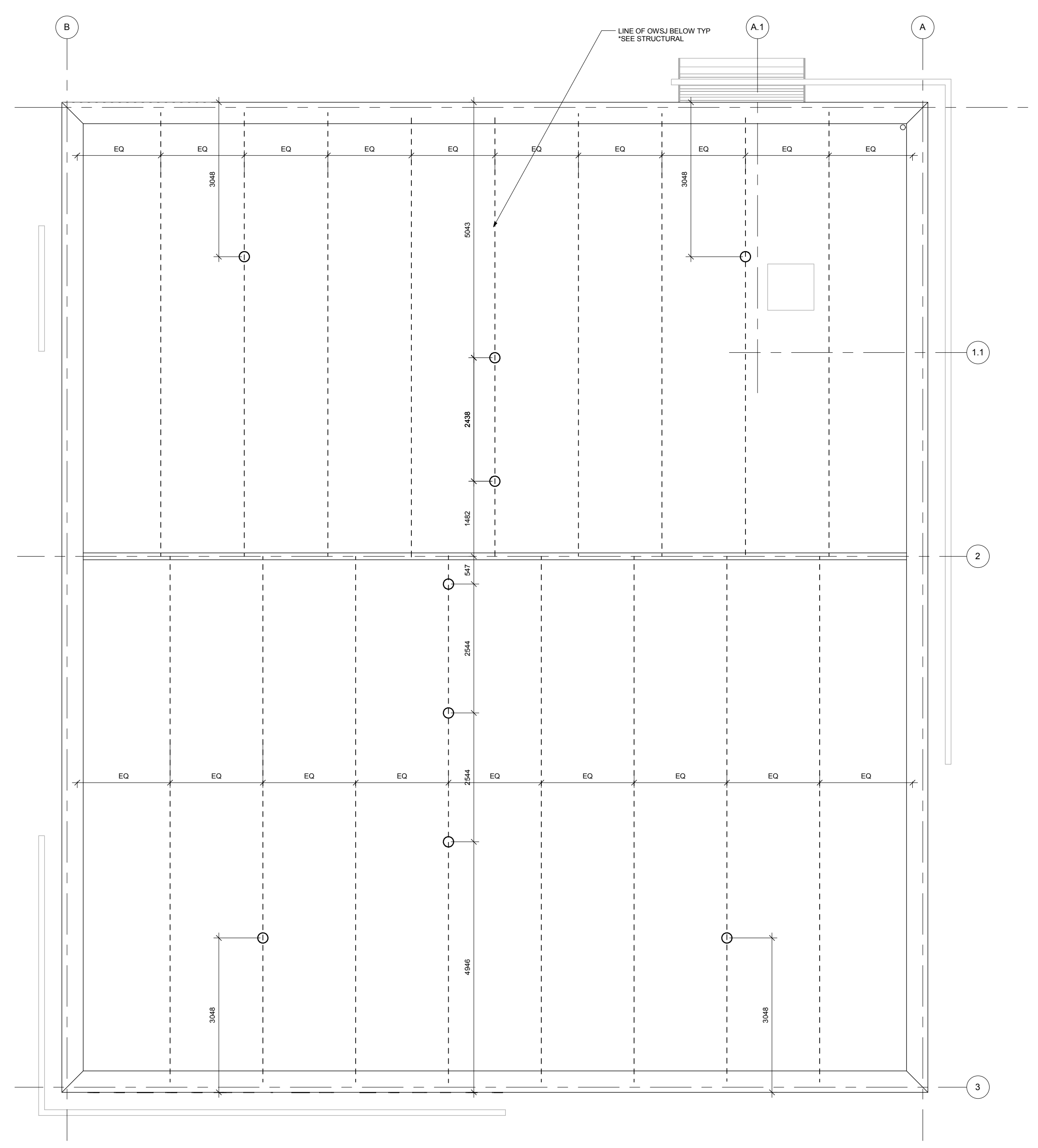
2 ROOF ANCHOR LOCATION SKETCH 1:50
