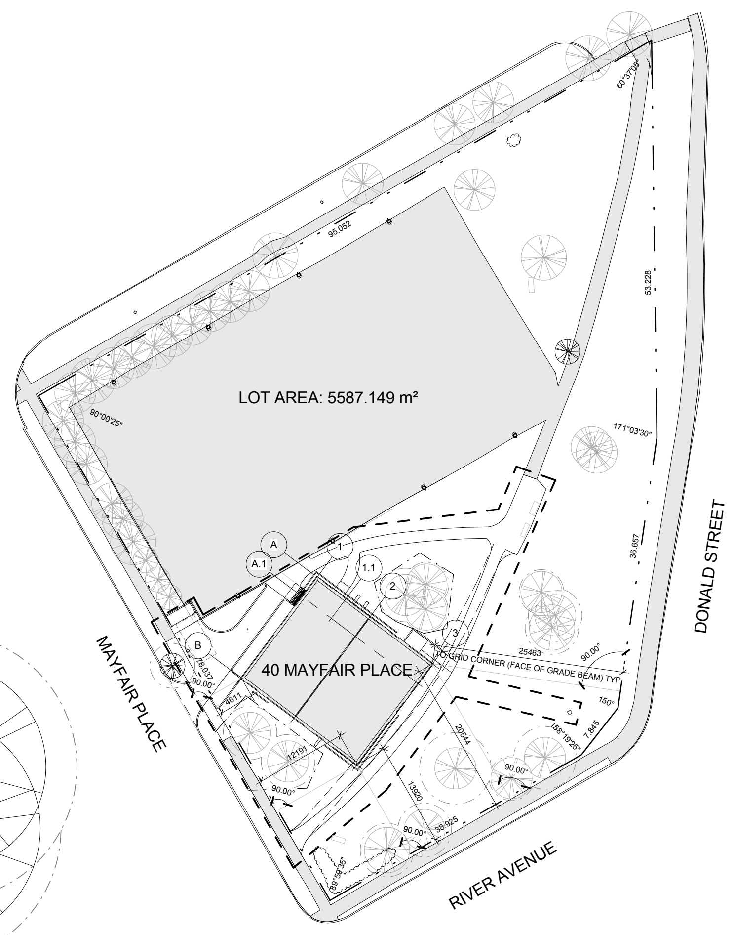
2 LOT DIMS/BLDG LOCATION 1:500
