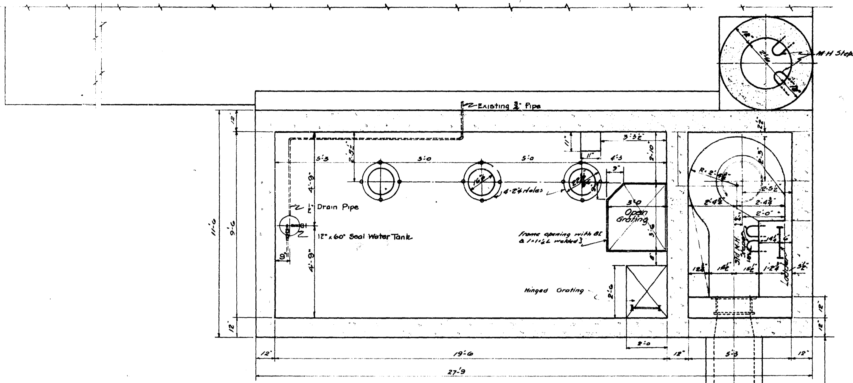
MOTOR FLOOR SECTION A-A
