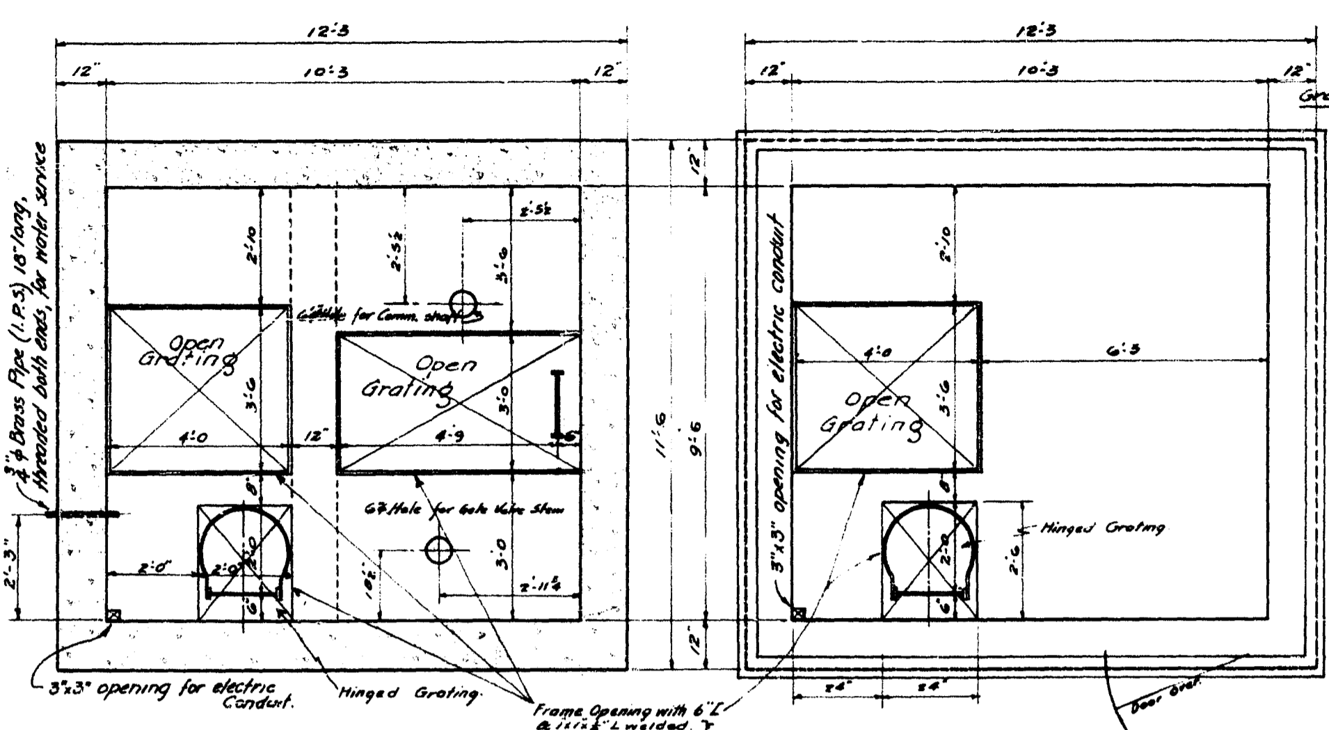
COMMINUTOR MOTOR FLOOR SECTION J-J GROUND FLOOR LEVEL SECTION K-K
