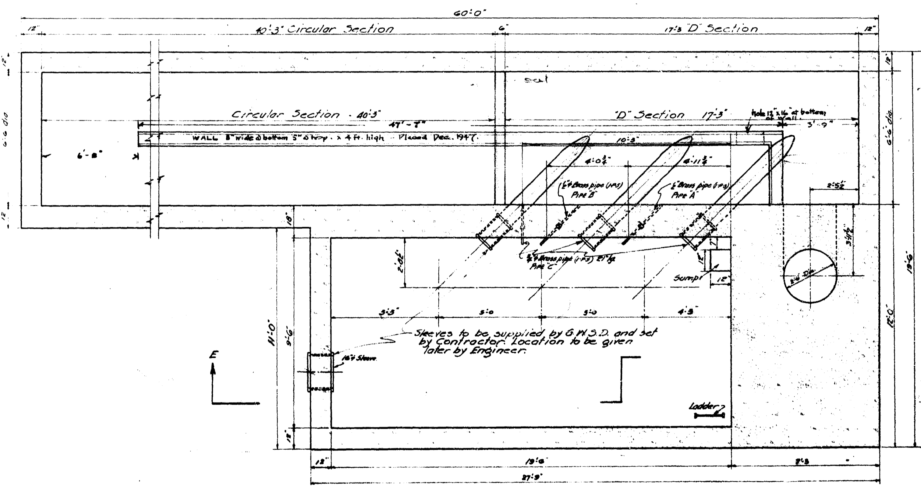
PUMP FLOOR SECTION B-B
