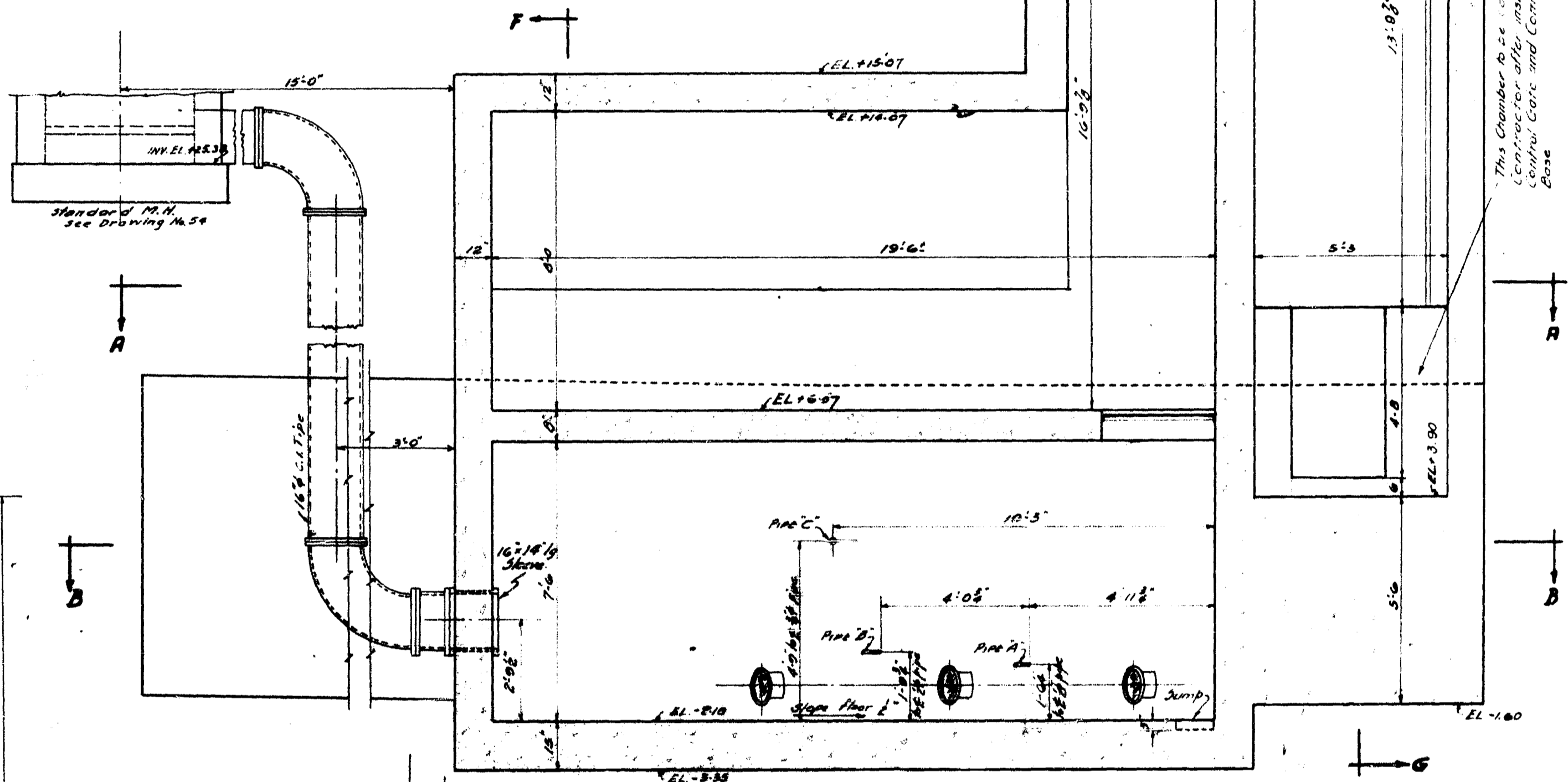
SECTION E-E
