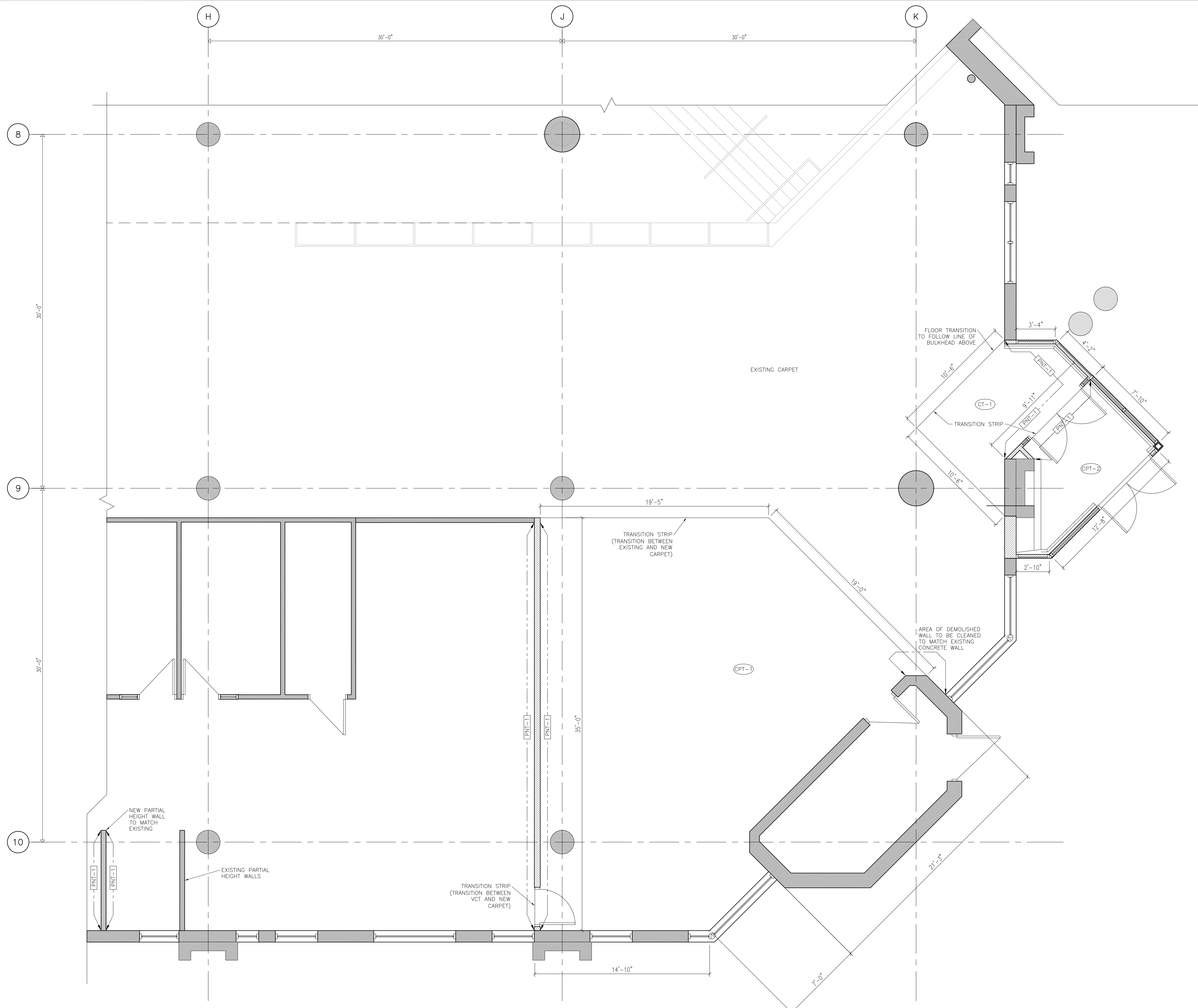
1 FINISH FLOOR PLAN 1/8" = 1'-0"
