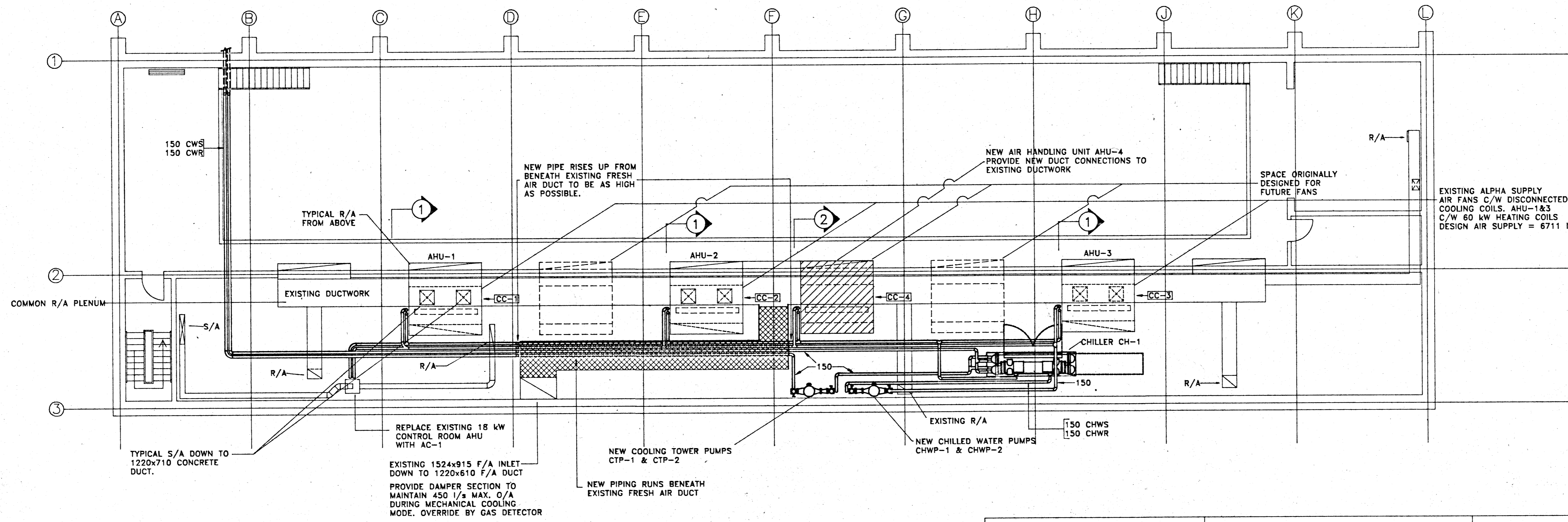
PLAN ABOVE ELEVATION 750.00
