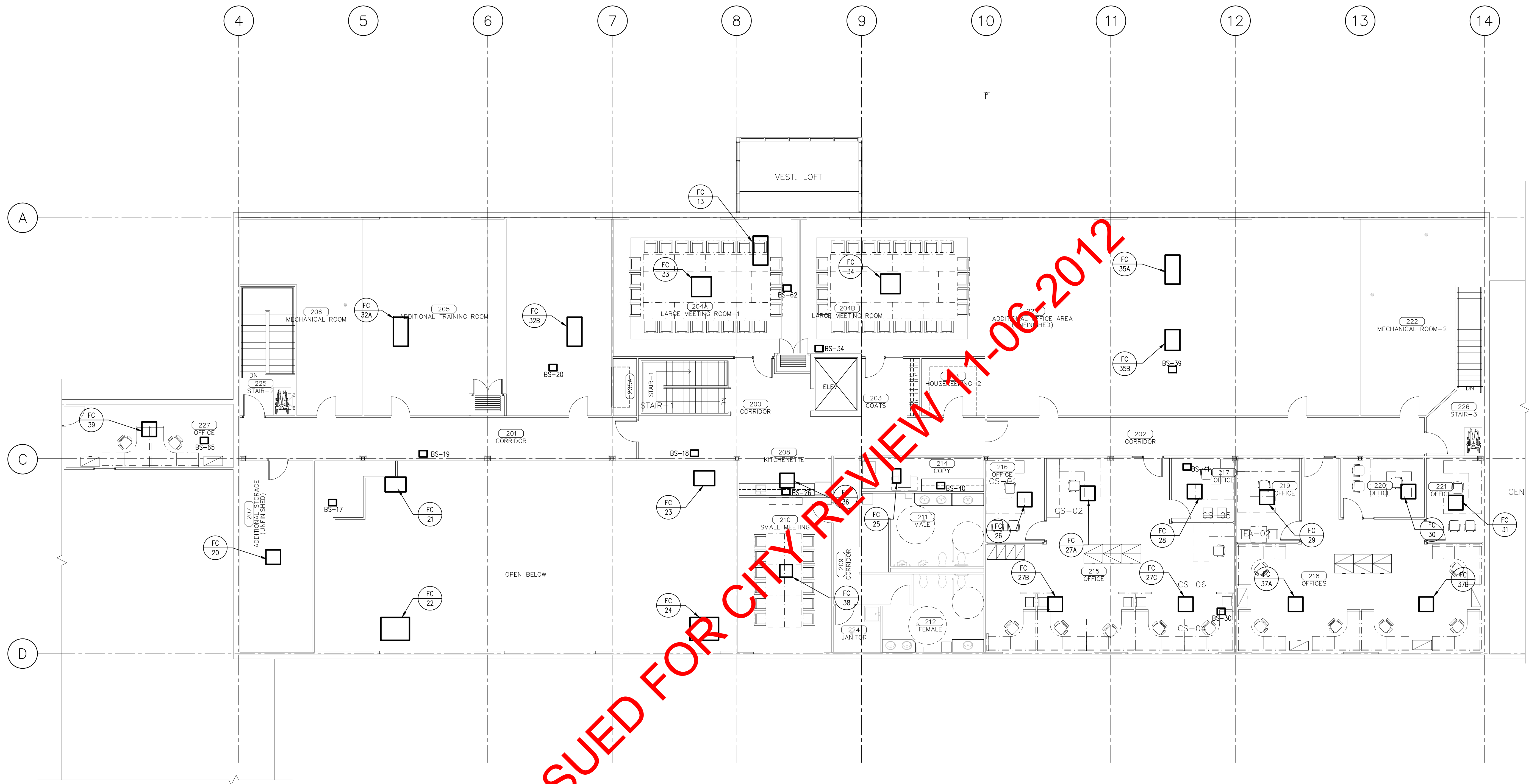
SECOND FLOOR PLAN - H.V.A.C. SCALE 1:100
