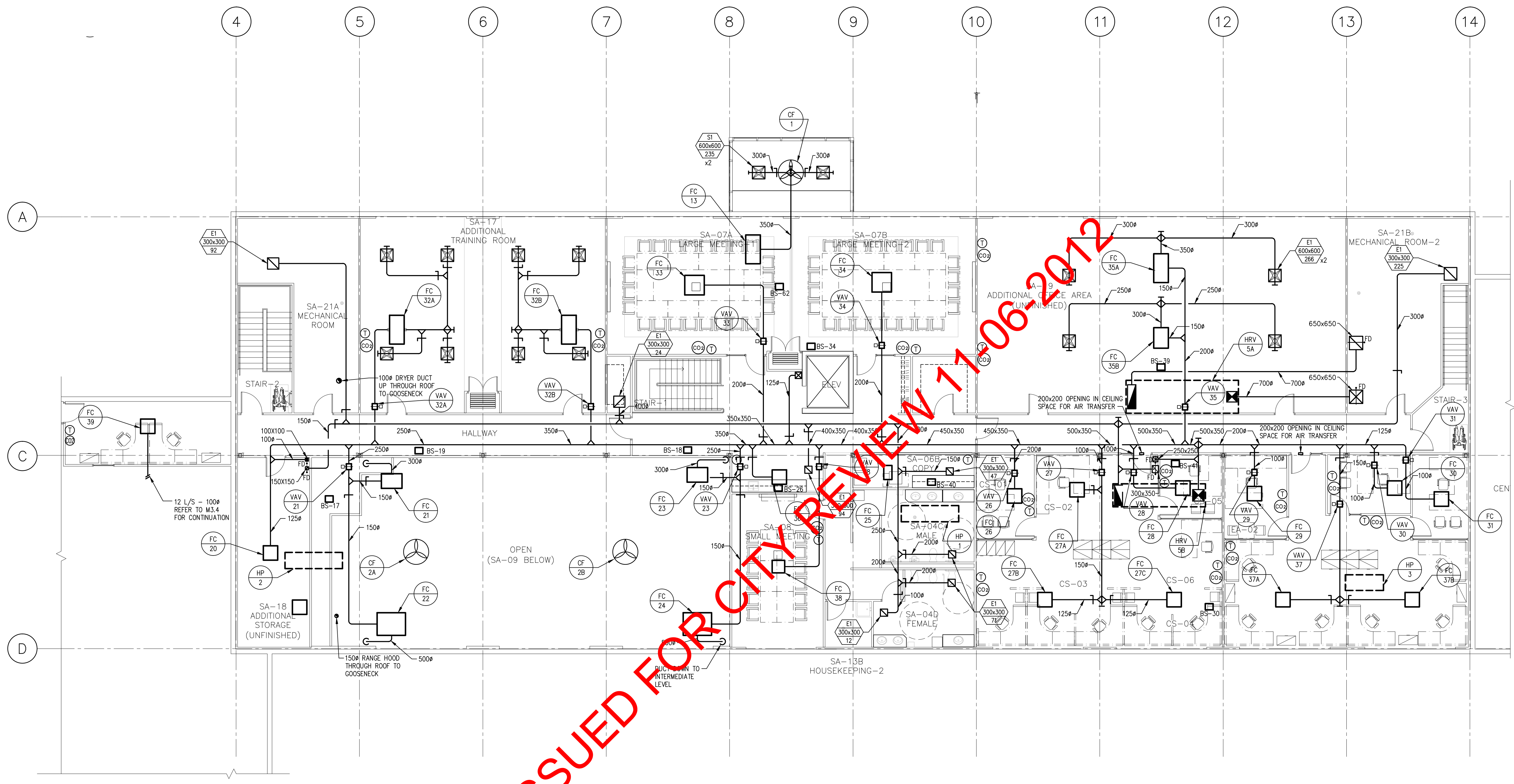
SECOND FLOOR PLAN - H.V.A.C. SCALE 1:100
