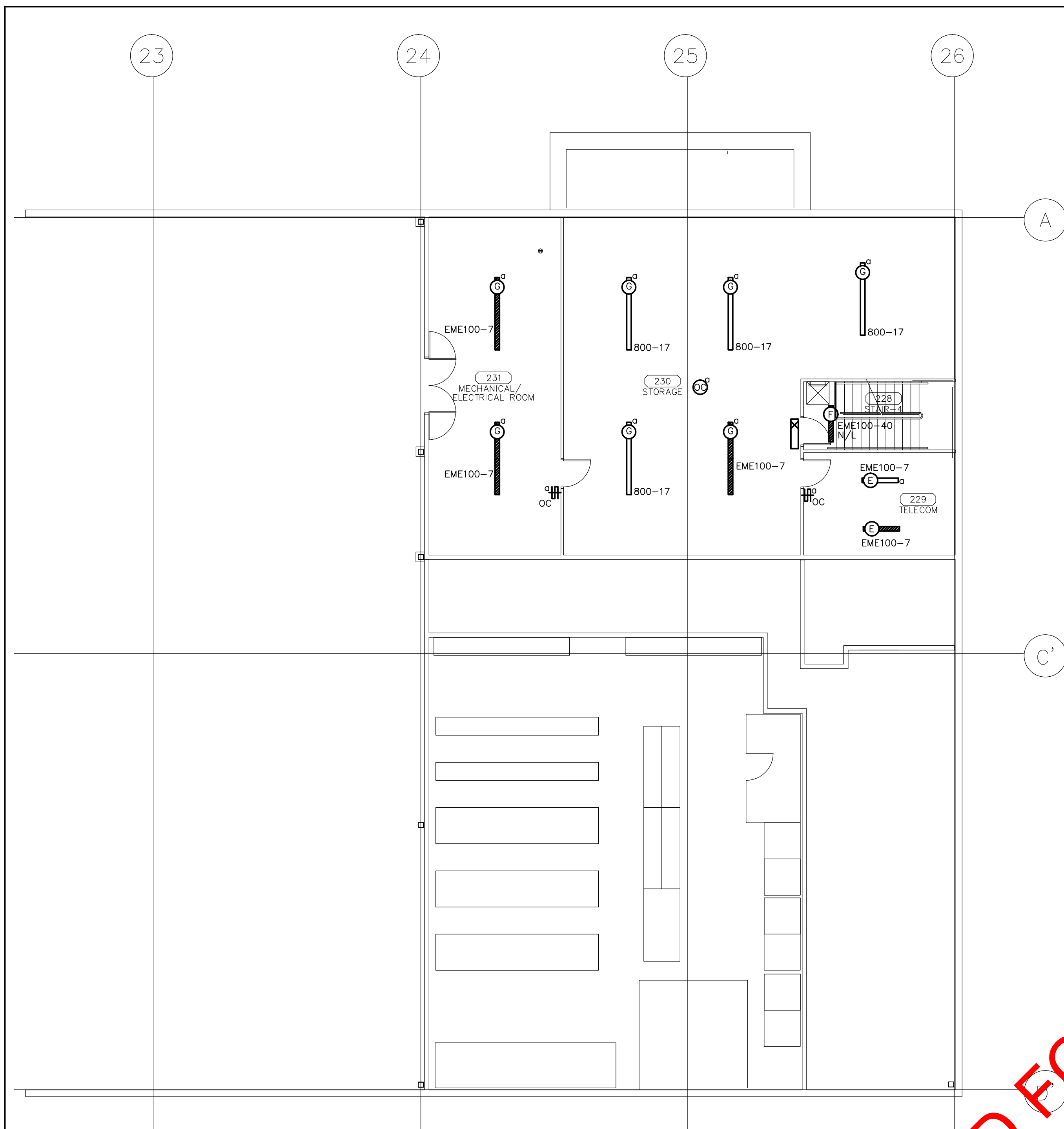
1 E2.5 PARTIAL SECOND FLOOR PLAN FLEET MANAGEMENT - LIGHTING LAYOUT SCALE: 1/100
