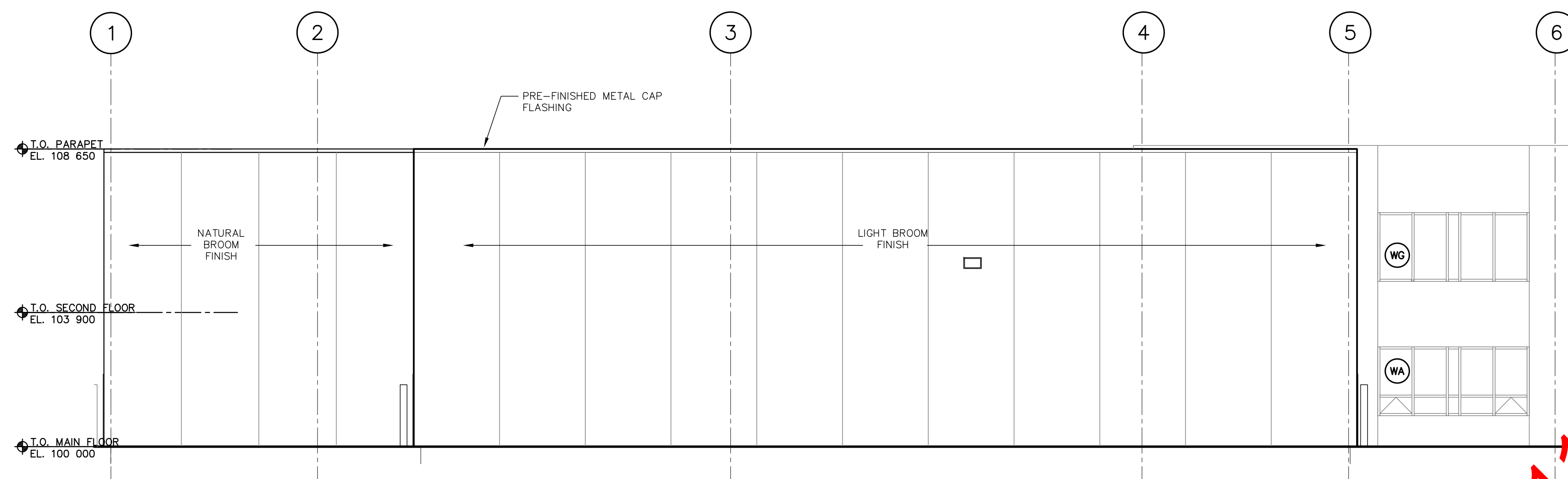
8 SOUTH BUILDING ELEVATION 4.5 SCALE 1:100
