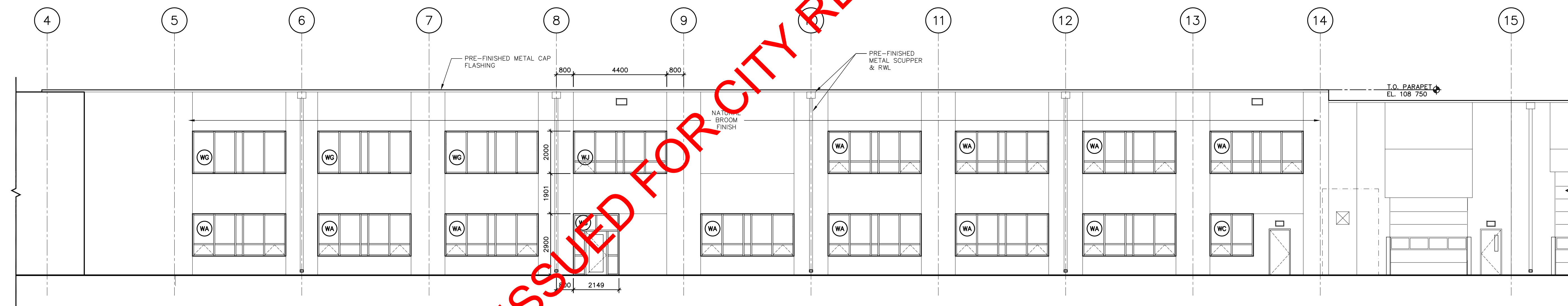
9 SOUTH BUILDING ELEVATION CONT. 4.5 SCALE 1:100
