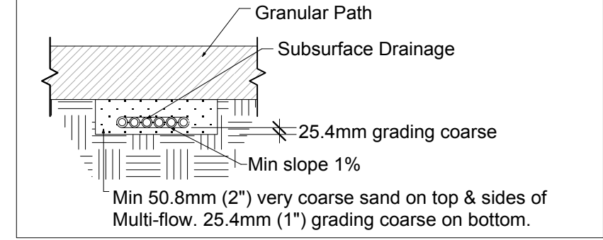
SUBSURFACE DRAINAGE UNDER PATH - NTS
