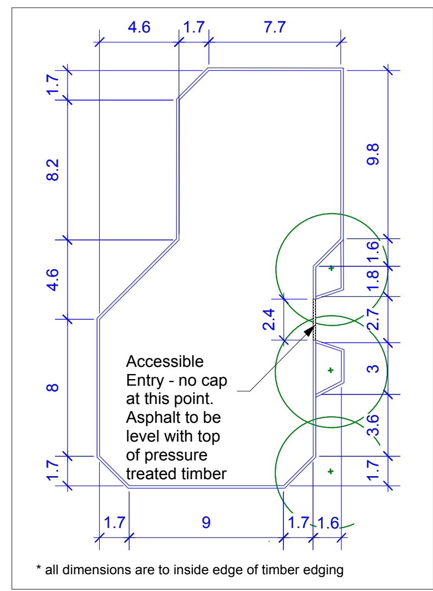
LAYOUT OF TIMBER EDGING - NTS
