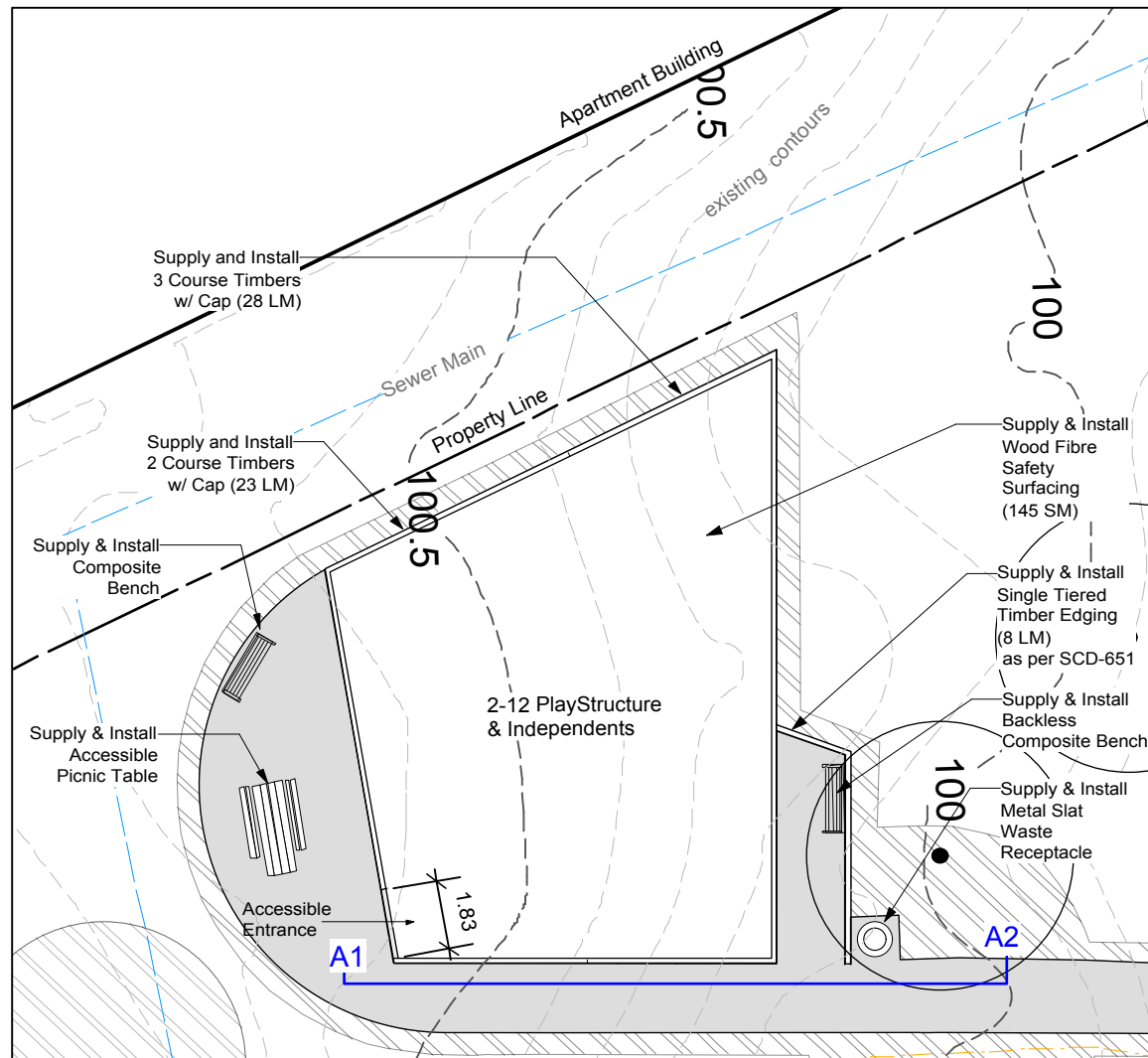
PLAY AREA PLAN Scale - 1:200
