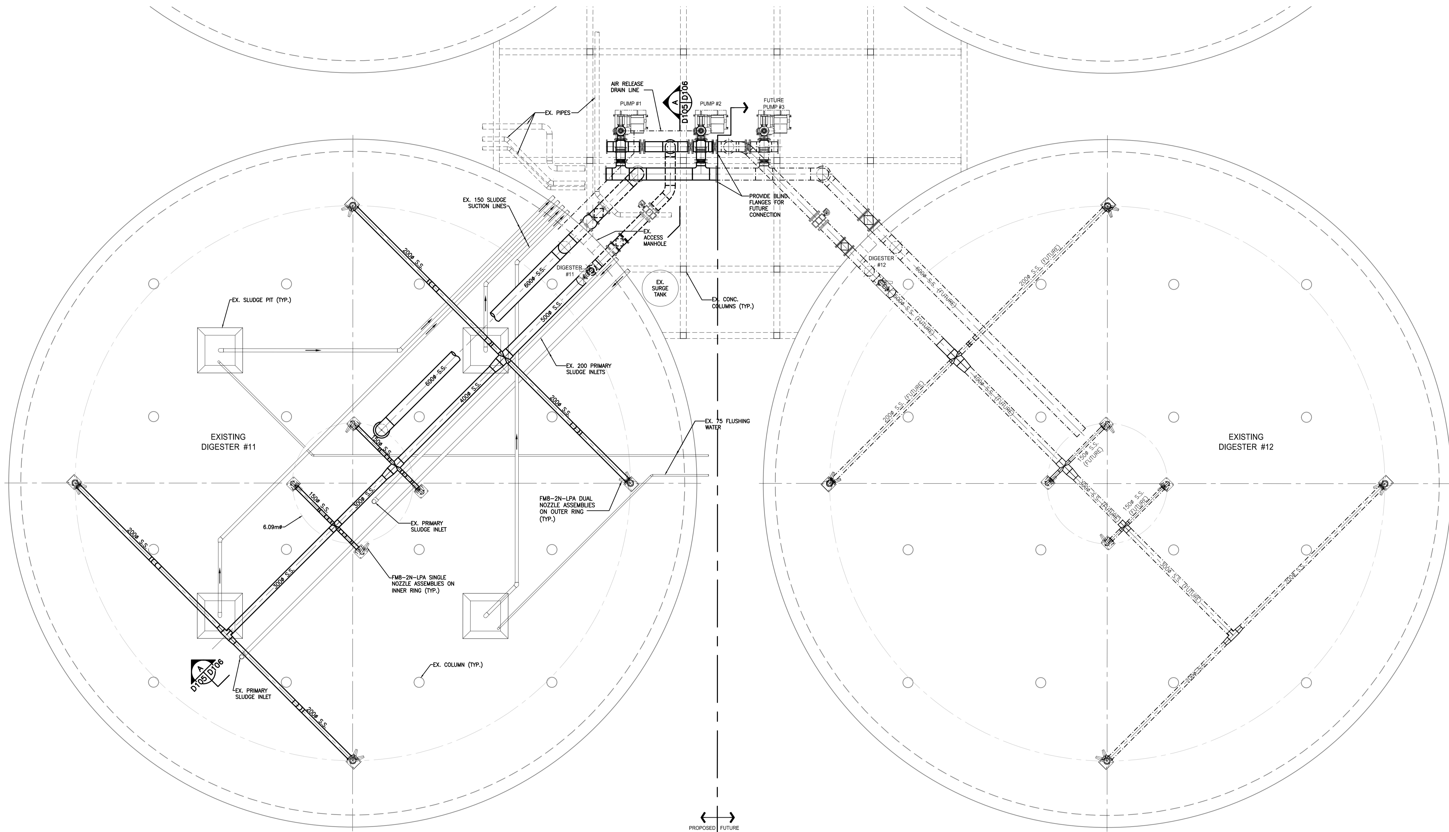
1 FLOOR PLAN 1:100
