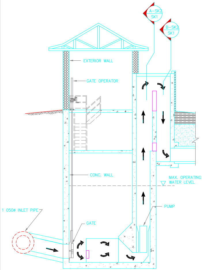
CROSS SECTION
