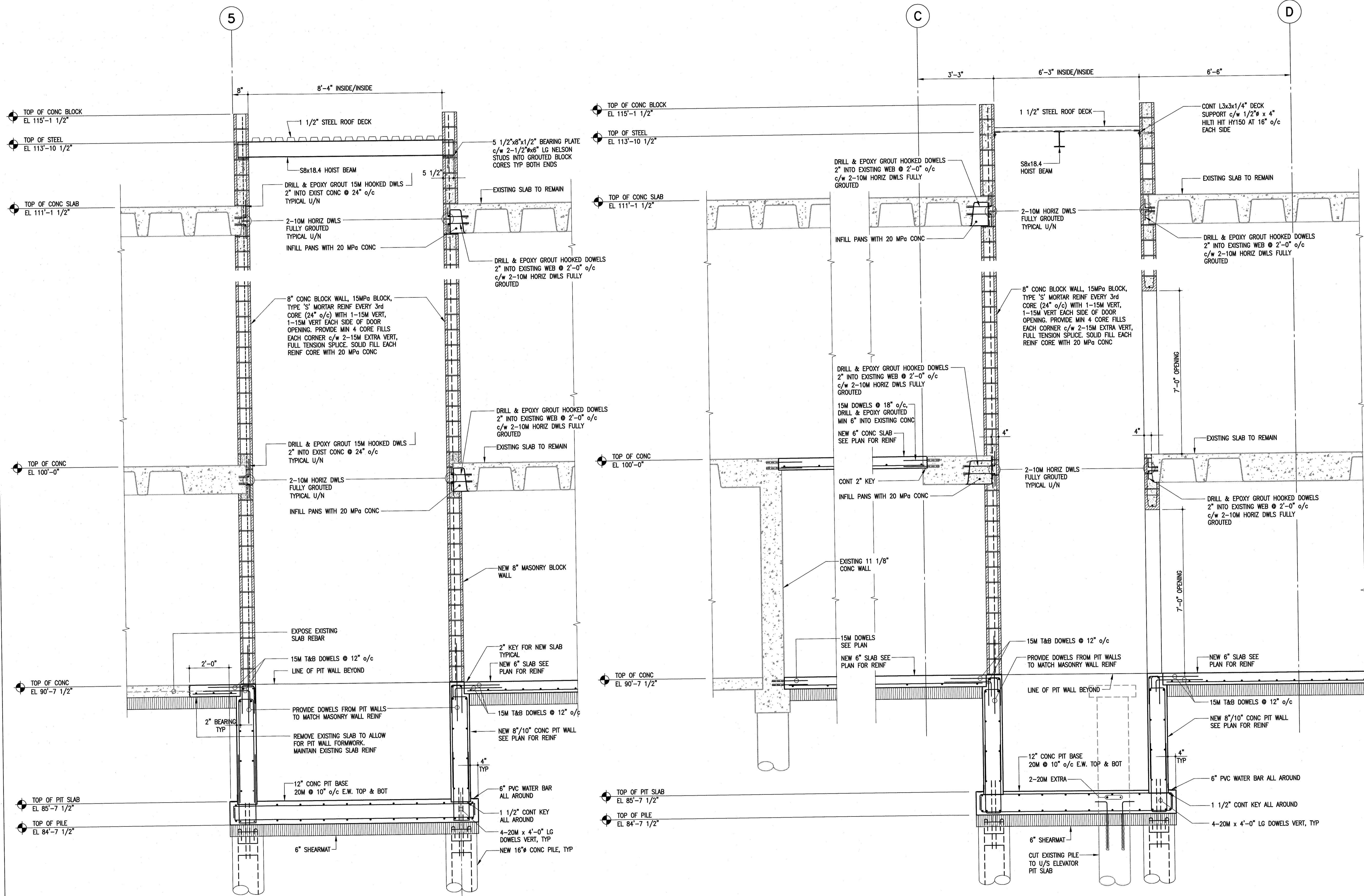
2 SECTION S2.1 1/2" = 1'-0"
