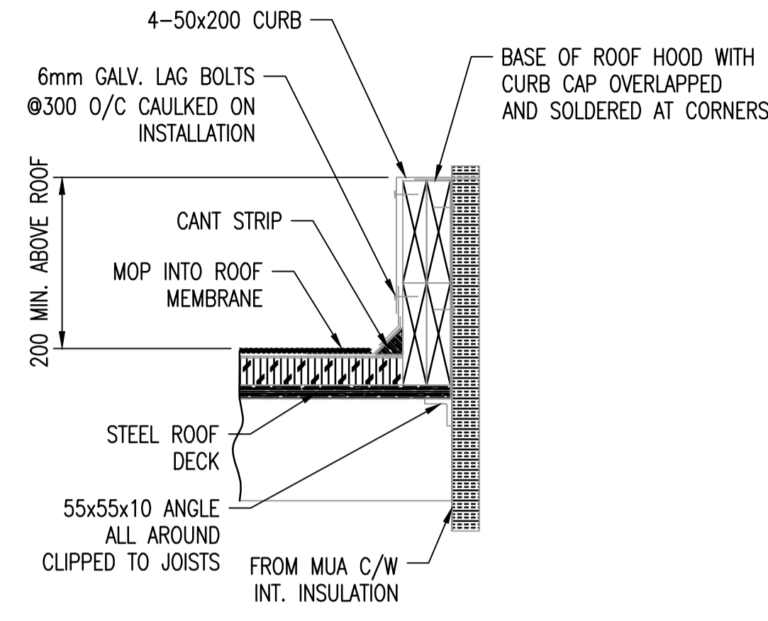
CURB DETAIL SCALE: NTS
