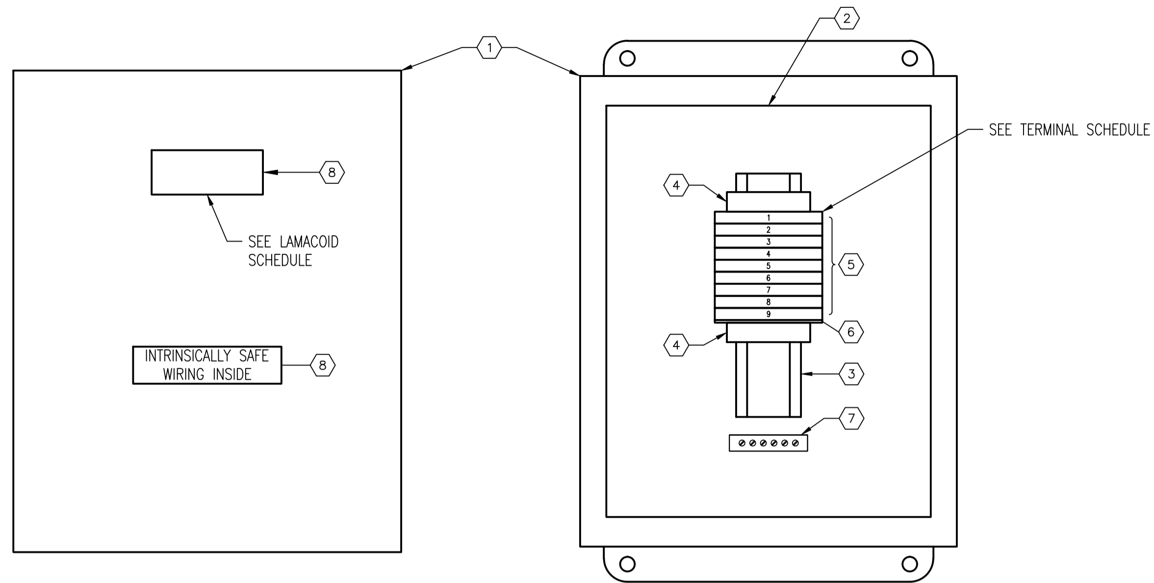
EXTERIOR PANEL VIEW SCALE: 1 : 2
