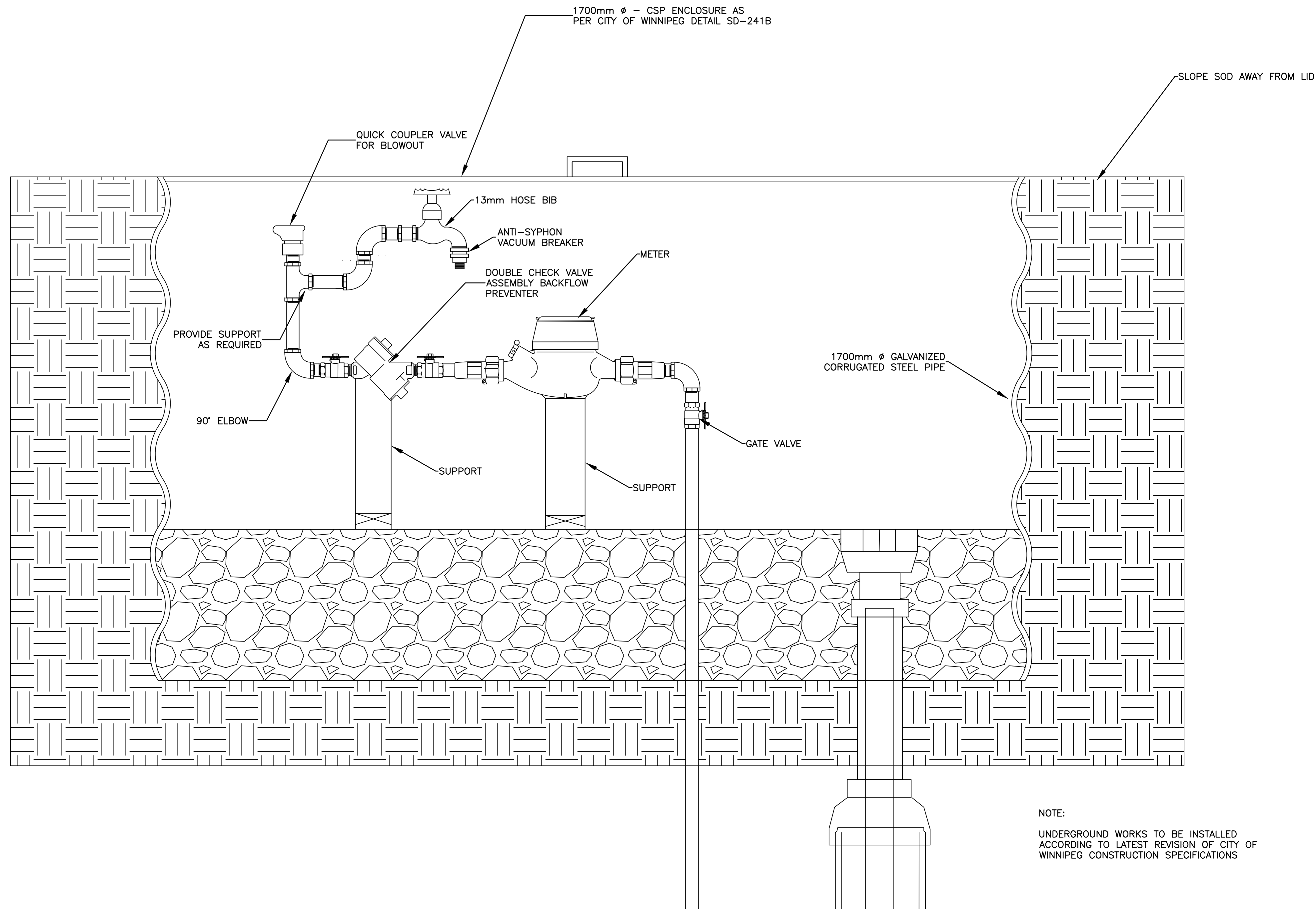
SECTION VIEW OF CSP ENCLOSURE SCALE= NTS
