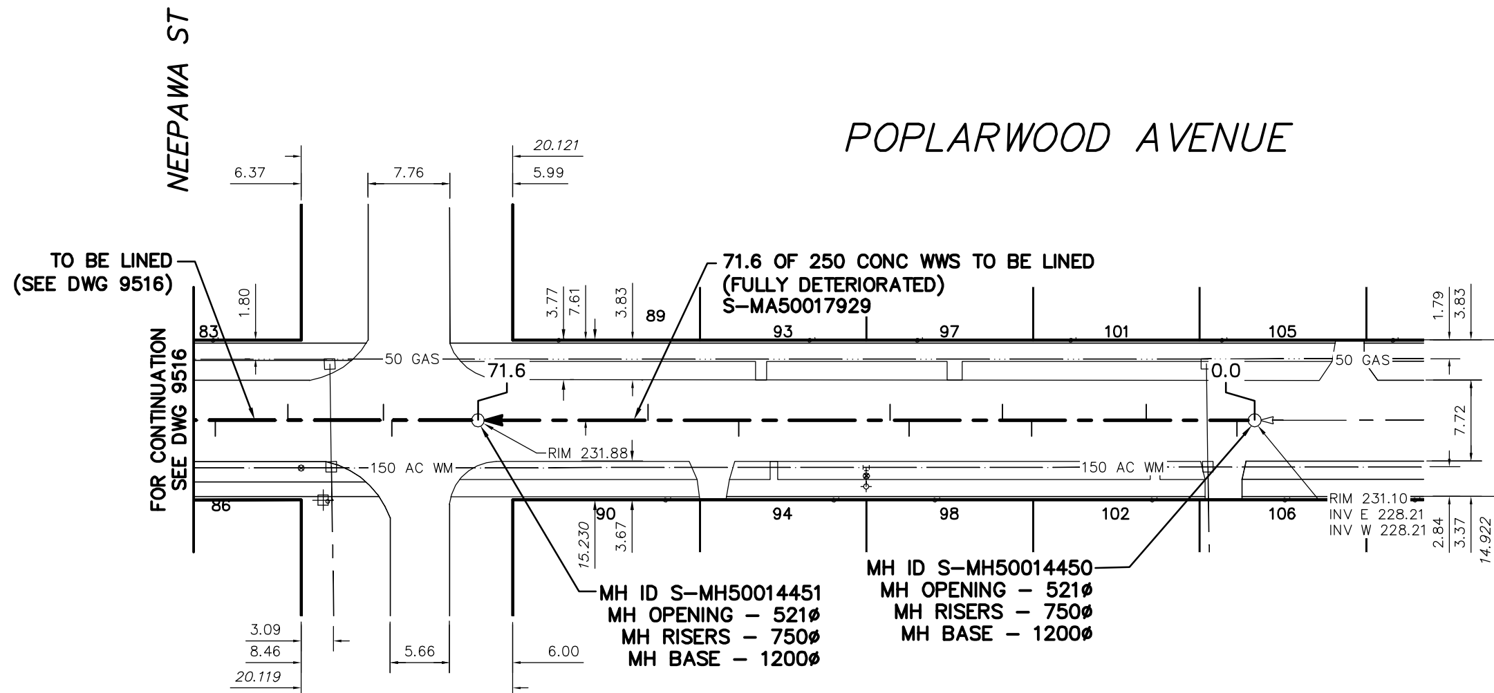
SEWER JUNCTION INFORMATION FROM SEWER VIDEO INSPECTION SEWER ID S-MA50017929
