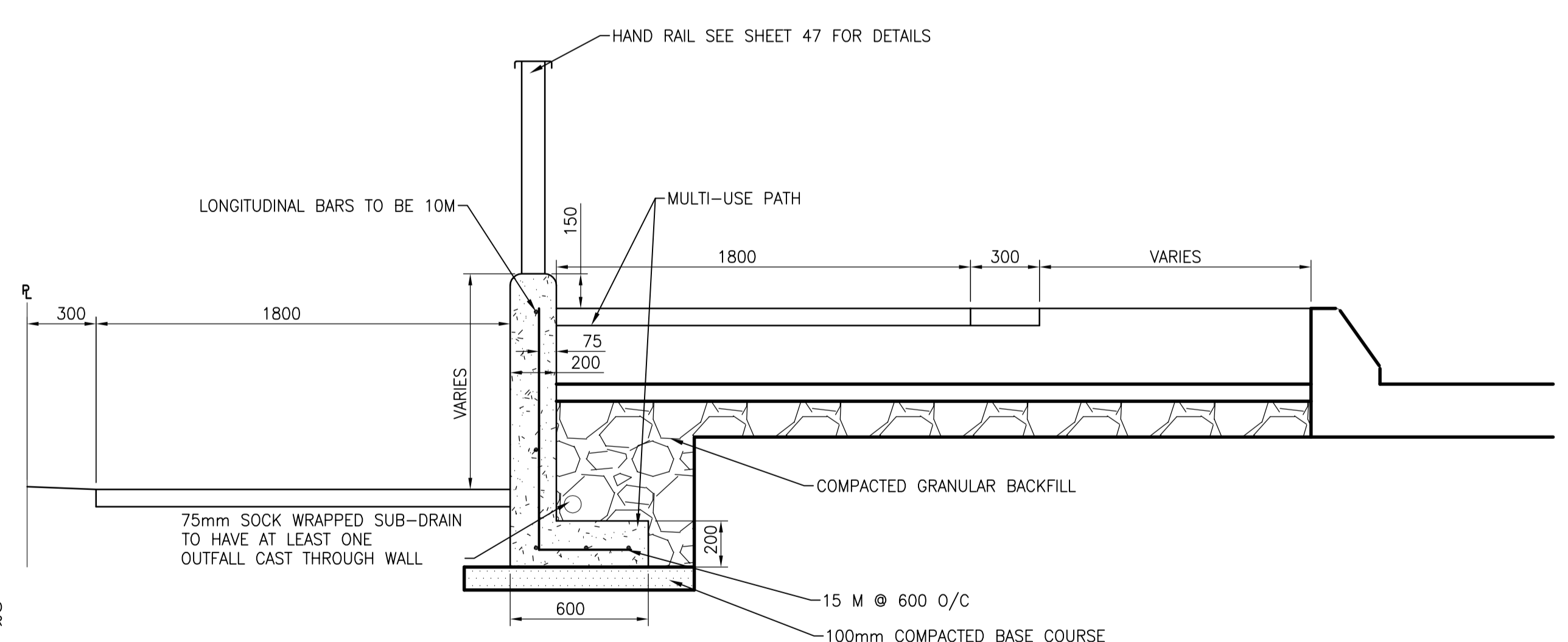
B SIDEWALK RETAINING WALL SECTION 1:20
