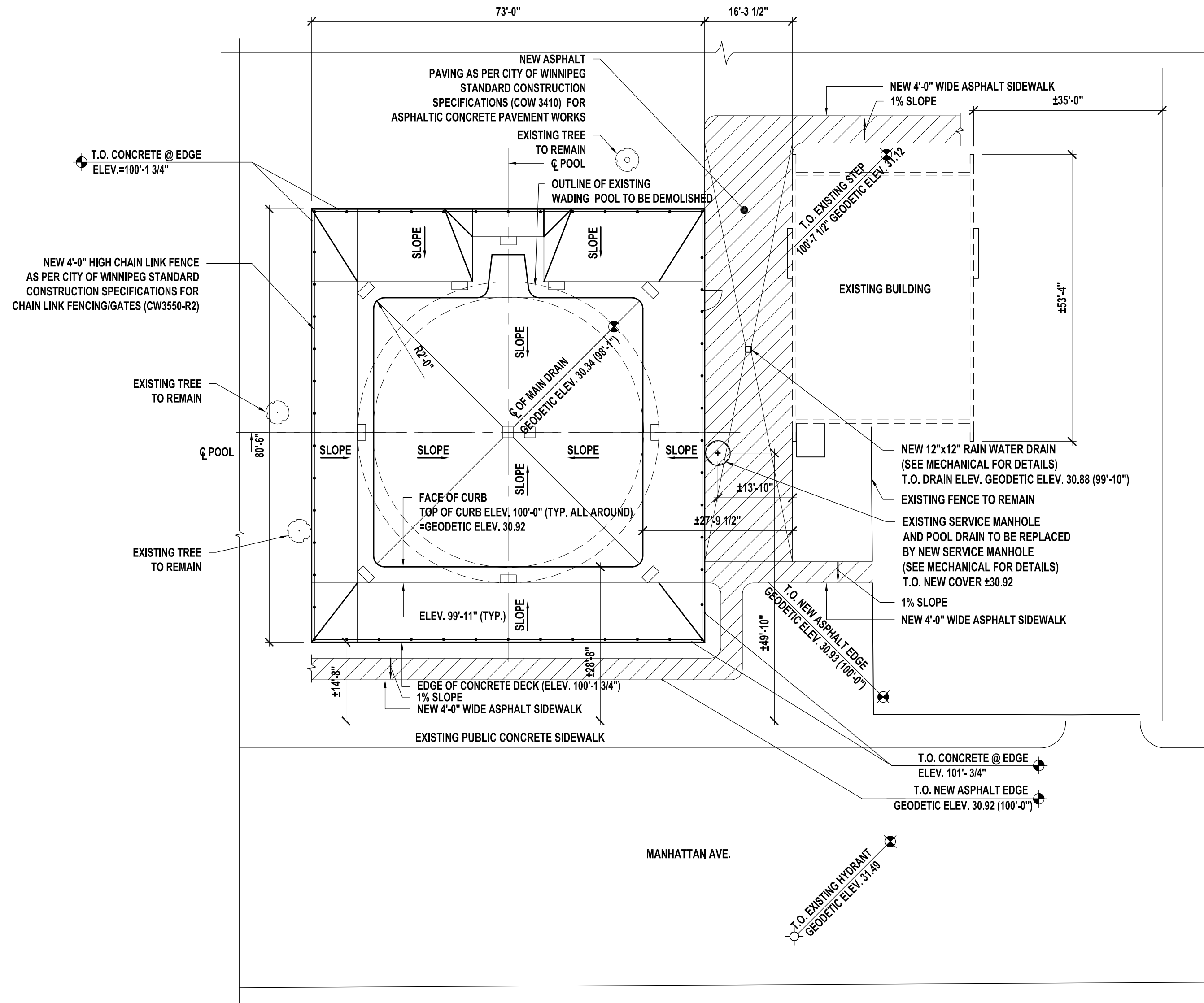
SITE PLAN Scale = 1/16" = 1'-0"
