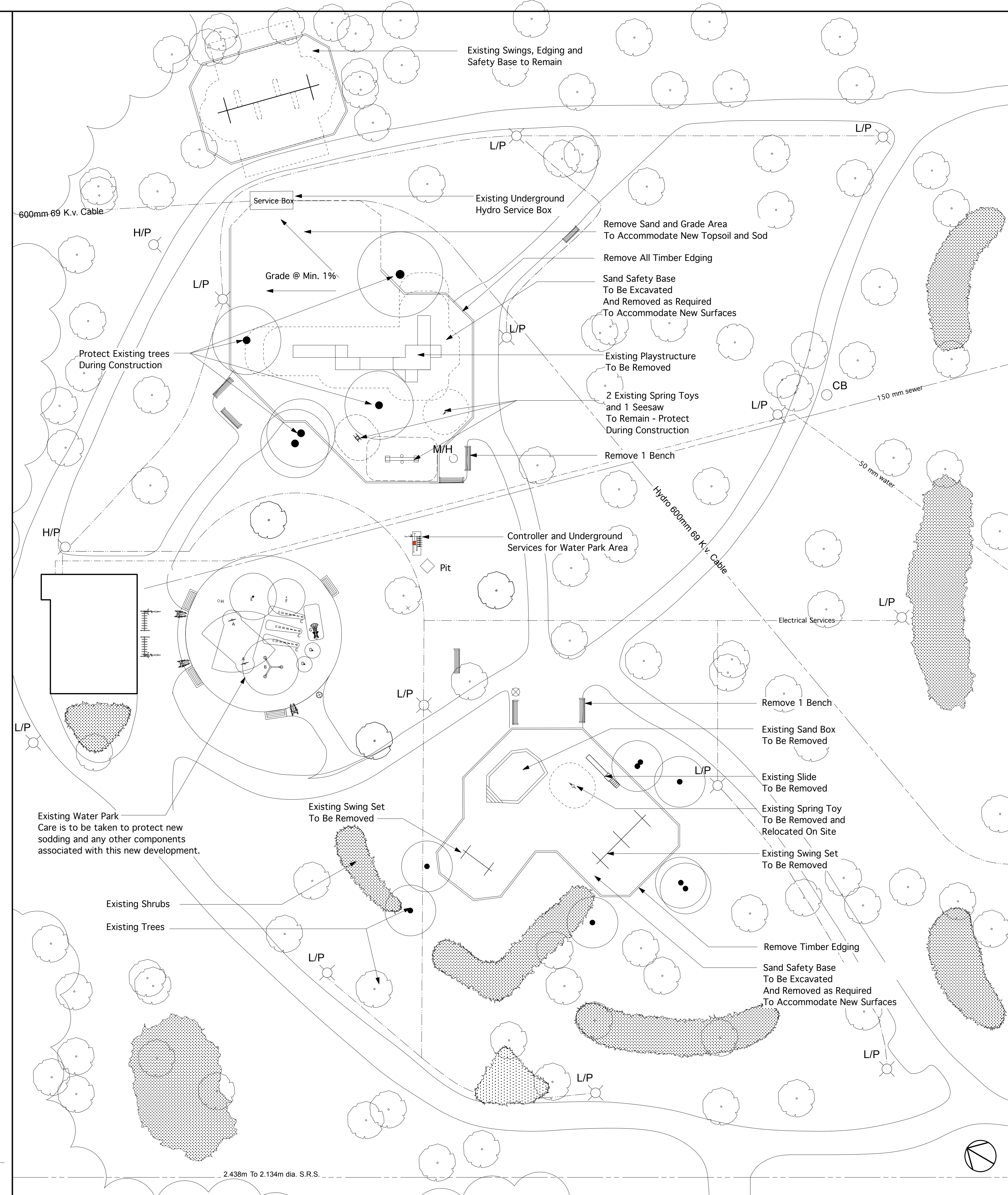
2 L1 EXISTING CONDITIONS AND REMOVALS PLAN Scale: 1:200
