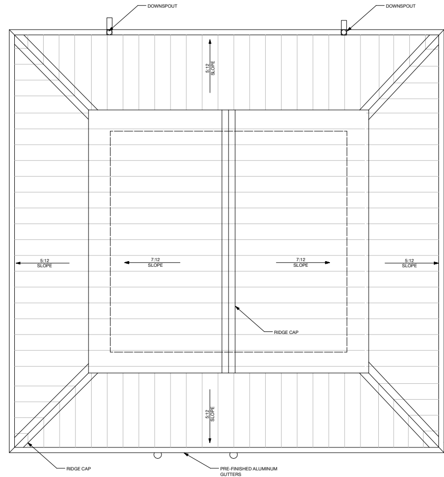
2 ROOF PLAN Scale: 1:25
