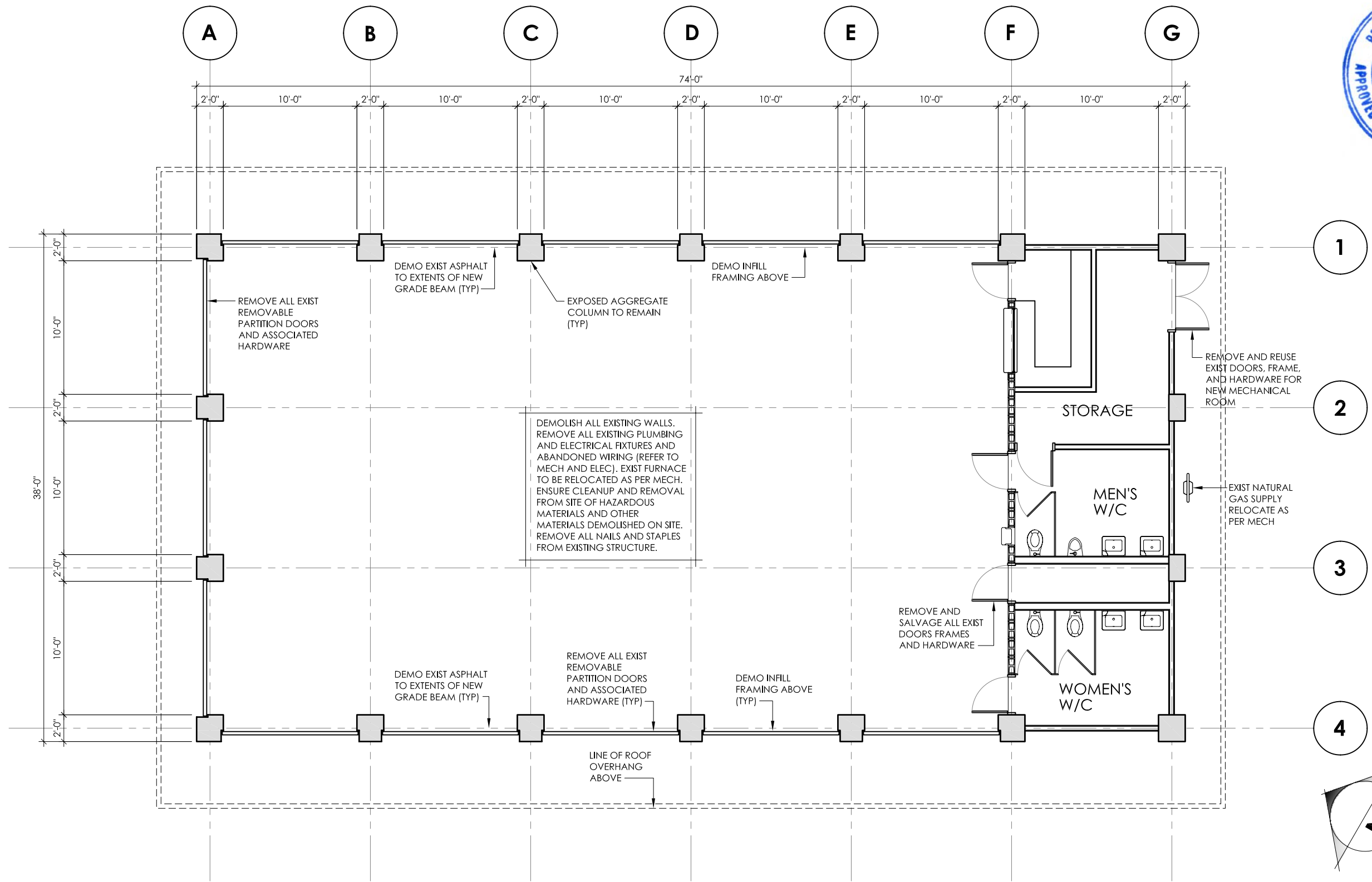
1 EXISTING FLOOR/DEMOLITION PLAN 1/8" = 1'-0"
