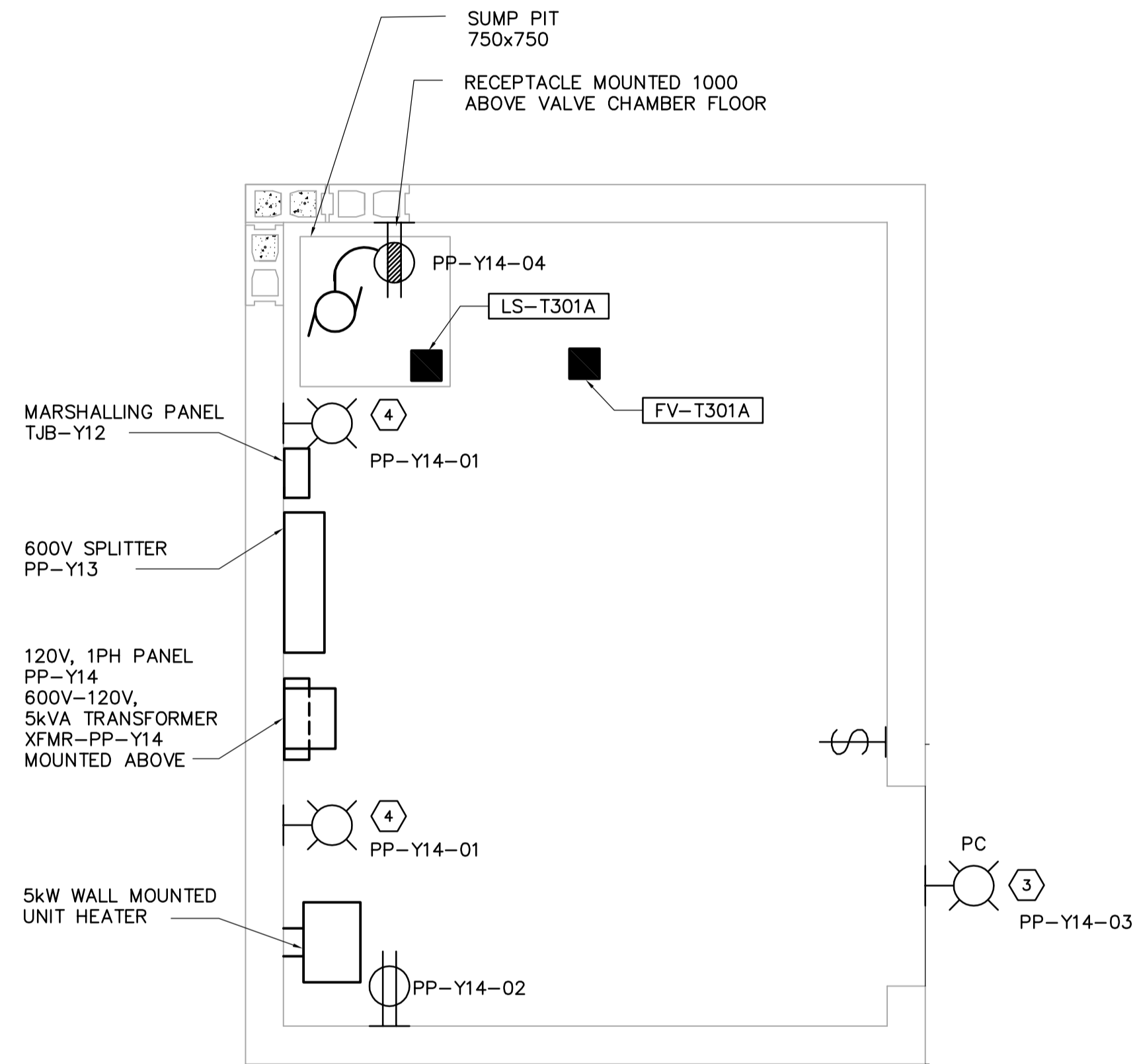
1 FLOOR PLAN 1:25
