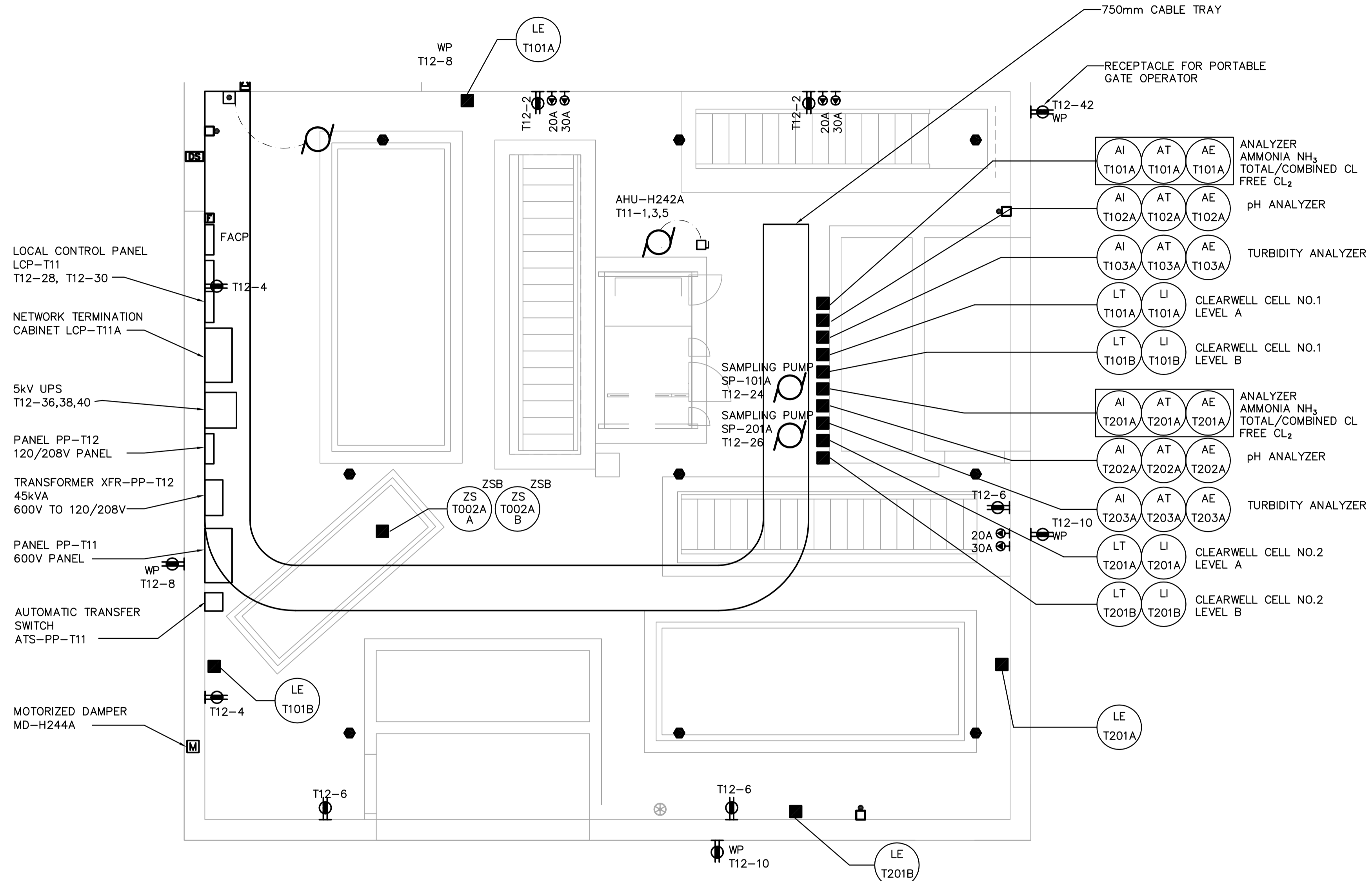
INLET BUILDING MAIN FLOOR POWER PLAN 1:50
