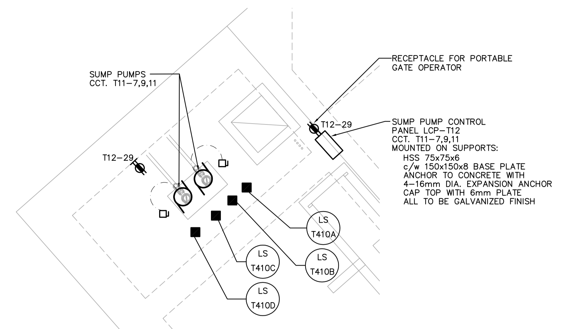
SUMP PIT AREA POWER PLAN 1:50
