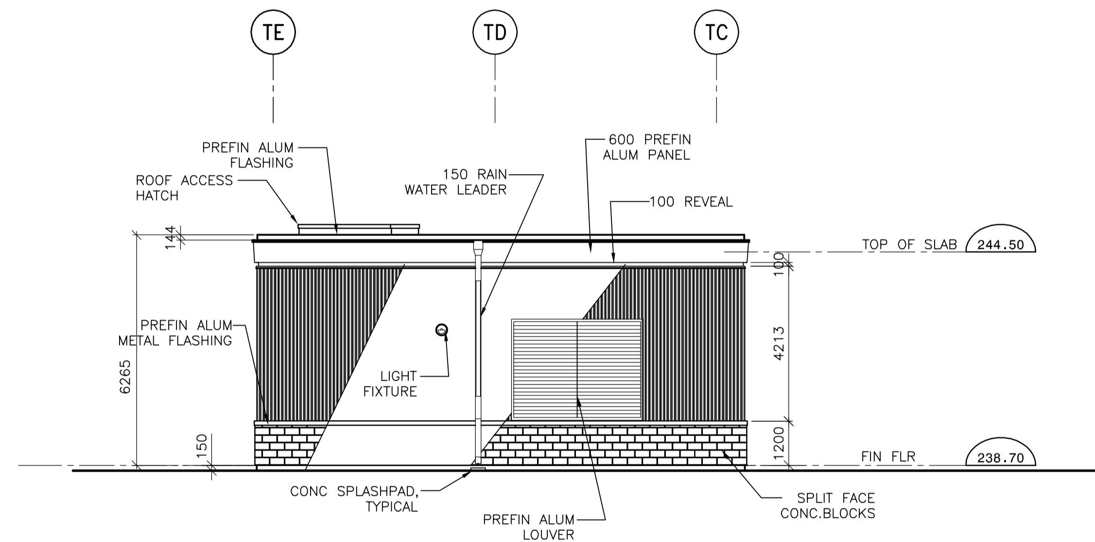
4 EAST ELEVATION 1:100
