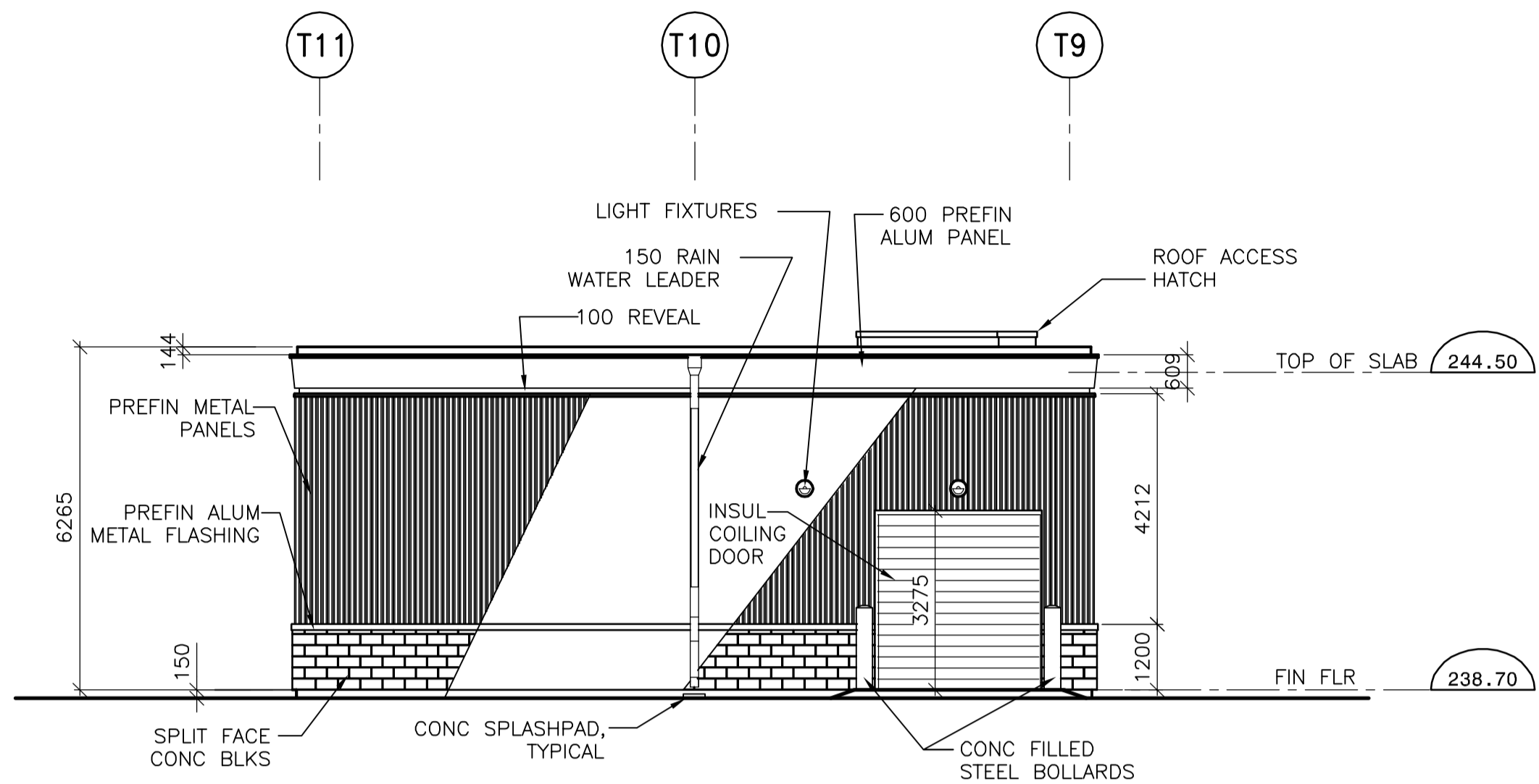
1 NORTH ELEVATION 1:100
