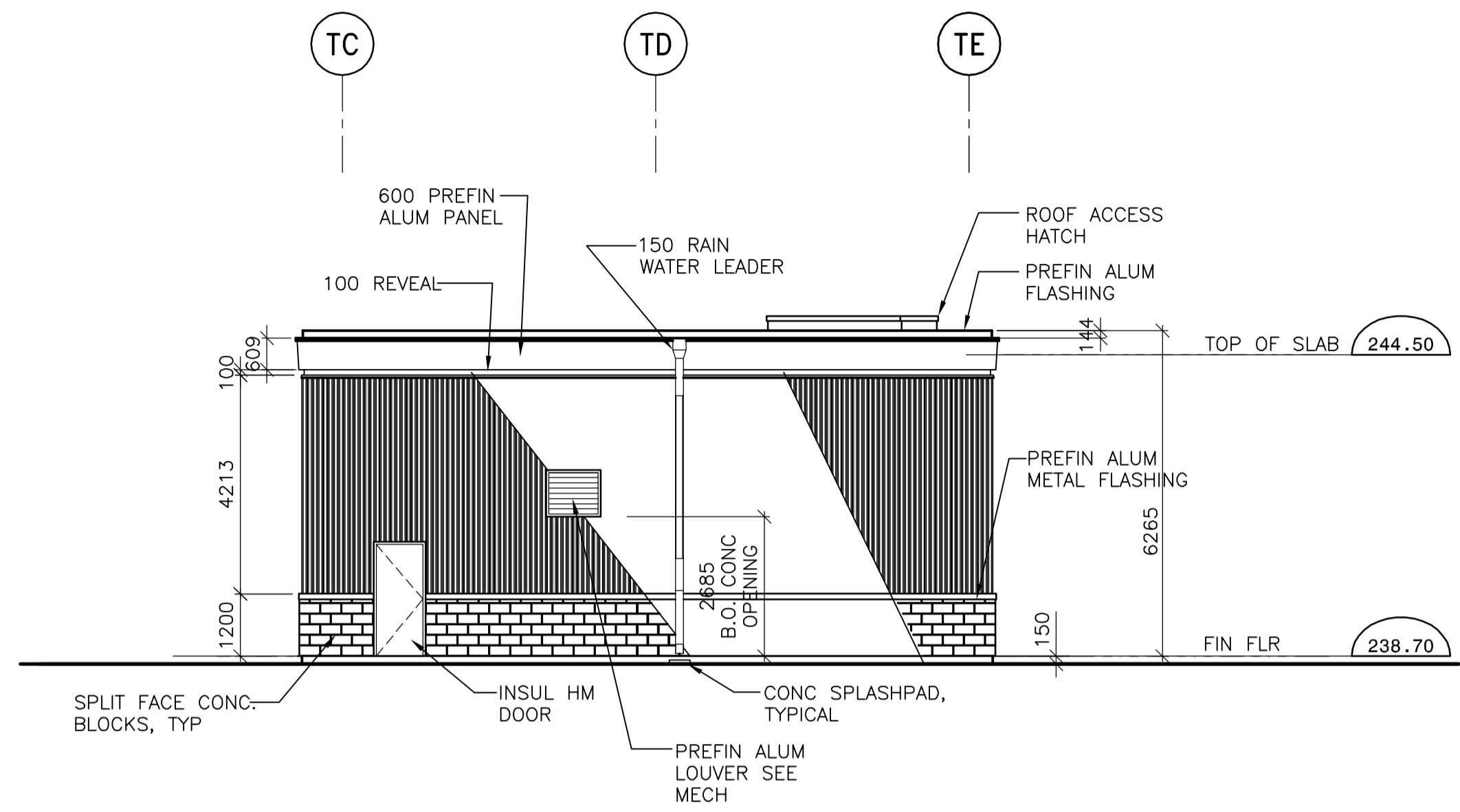
2 WEST ELEVATION 1:100
