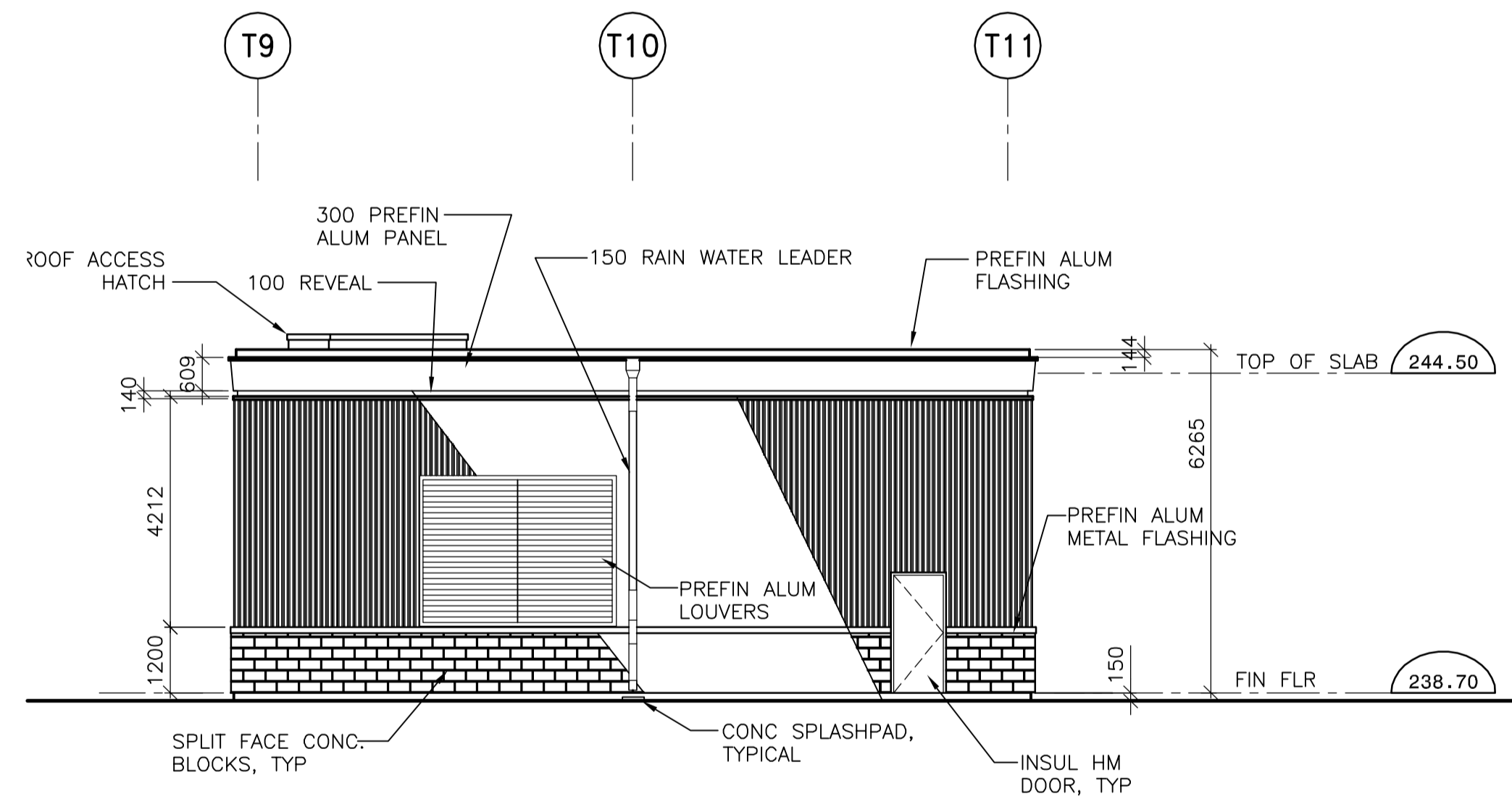
3 SOUTH ELEVATION 1:100
