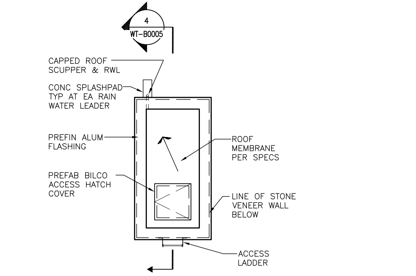
2 EMERGENCY EGRESS HUTS ROOF PLAN - TYPICAL OF 4 1:50
