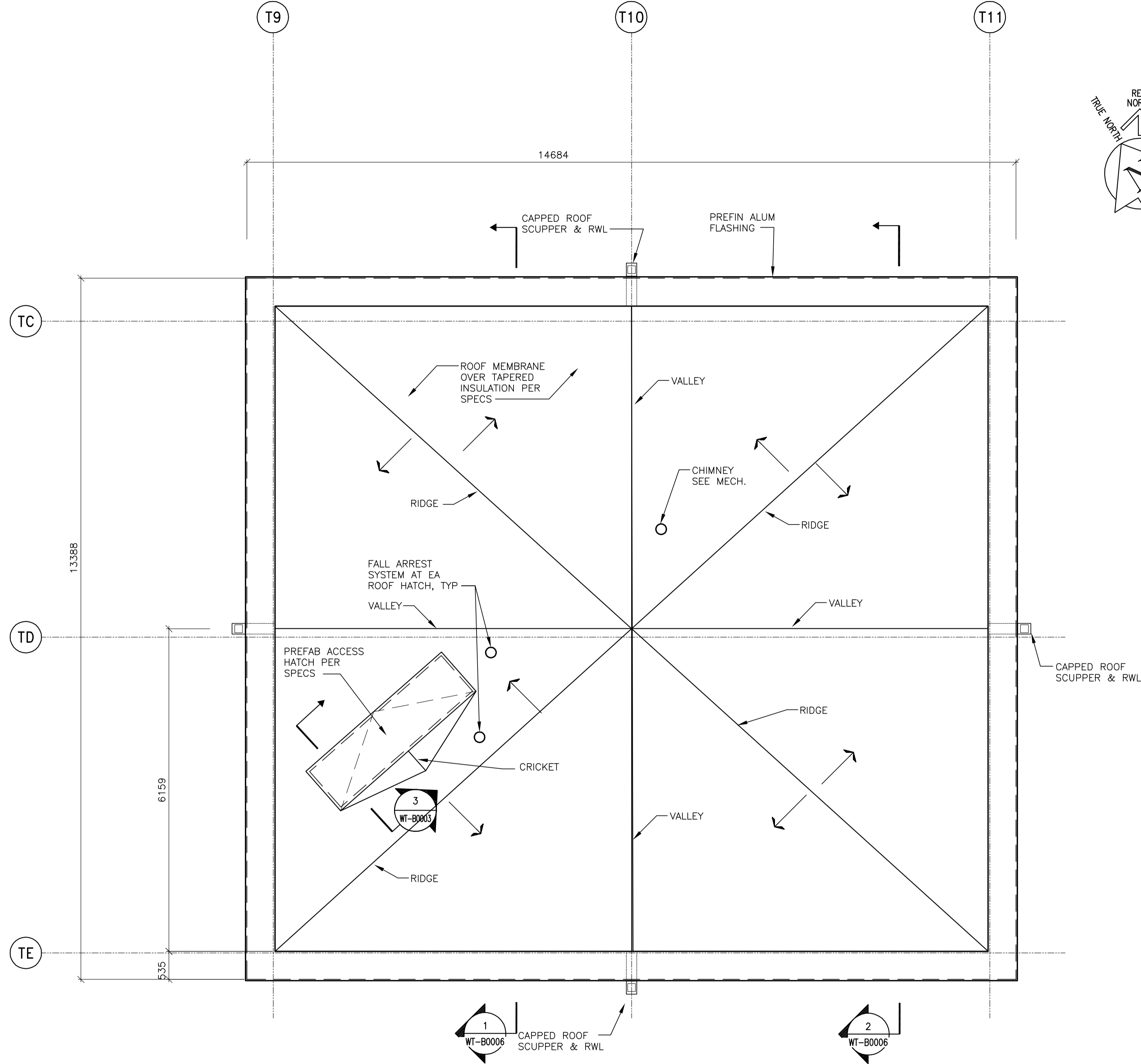
1 INLET BUILDING ROOF PLAN 1:50
