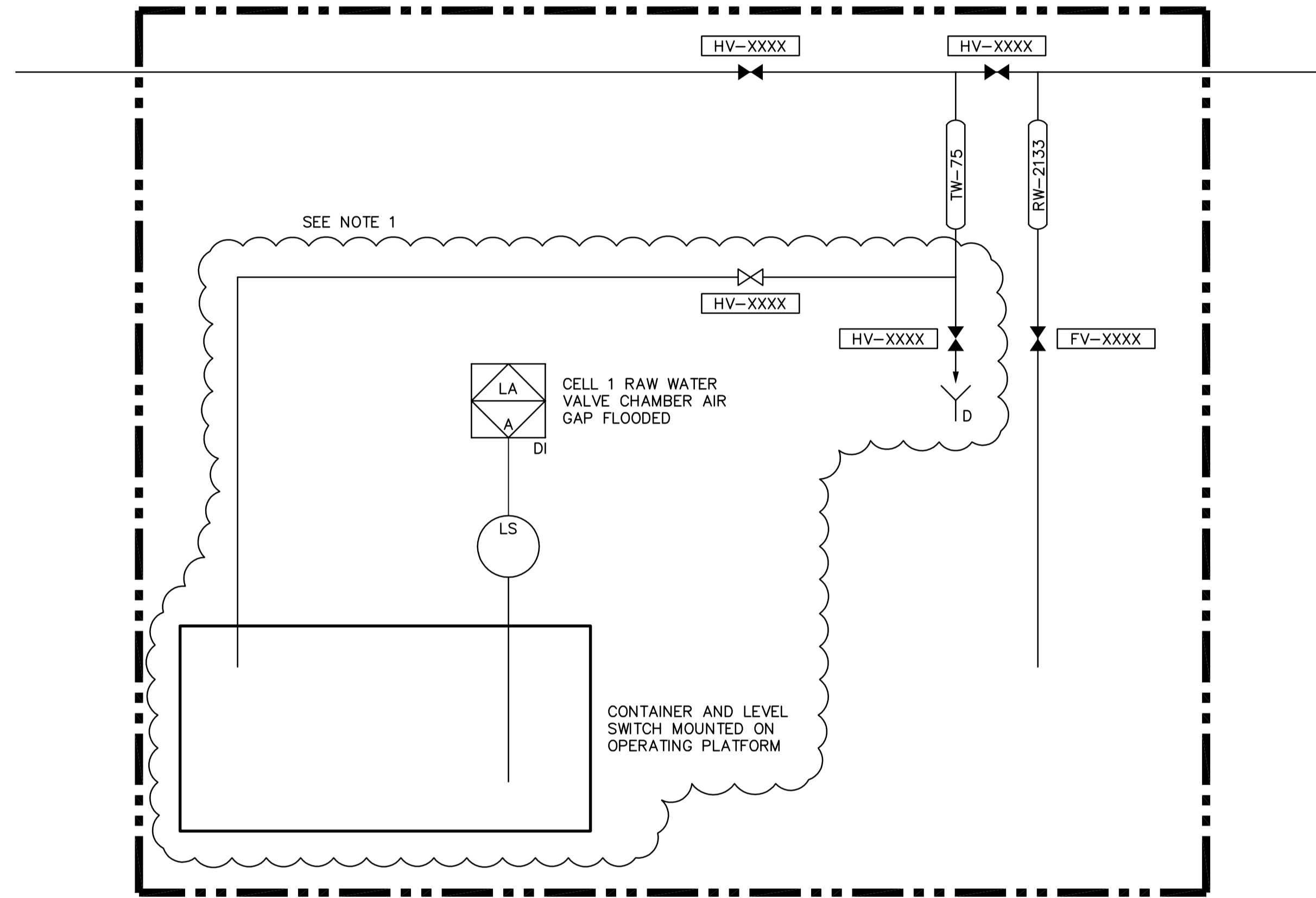
CELL 1 RAW WATER VALVE CHAMBER ALL TAG NUMBERS TO BE CONFIRMED
