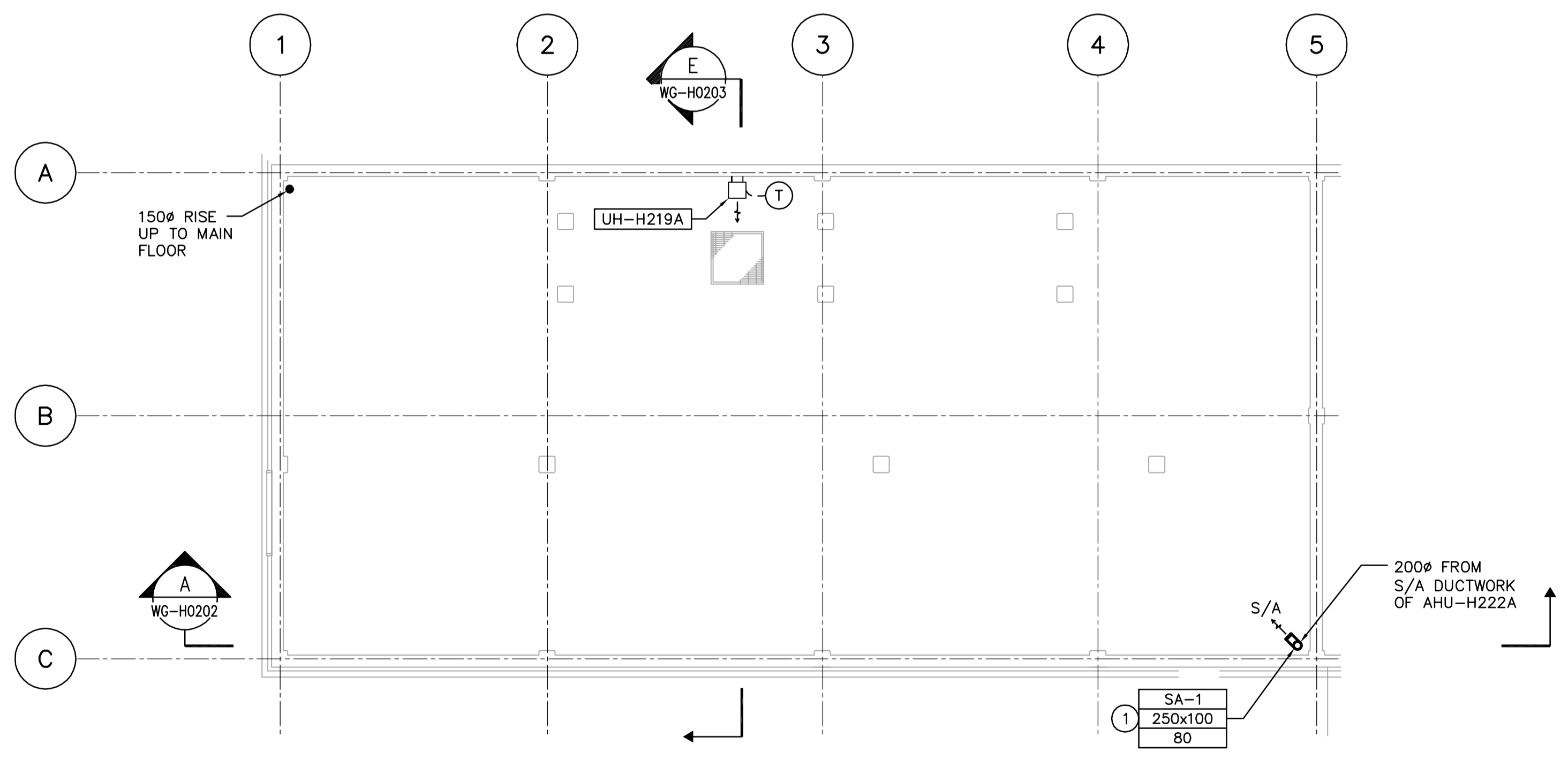
2 CRAWL SPACE VENTILATION PLAN 1:100
