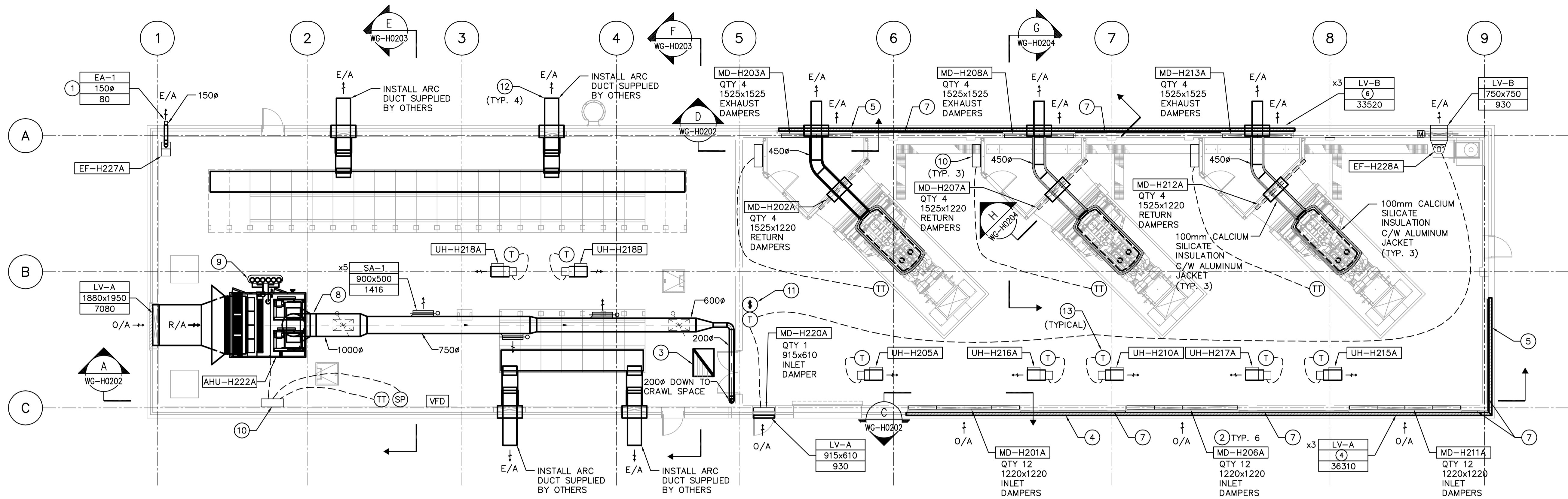
1 MAIN FLOOR VENTILATION PLAN 1:100
