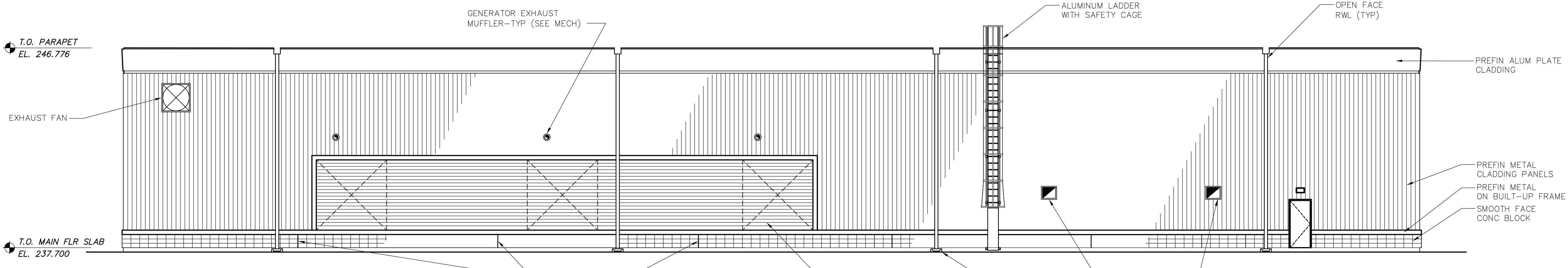
2 NORTH ELEVATION WG-B0301 1:100
