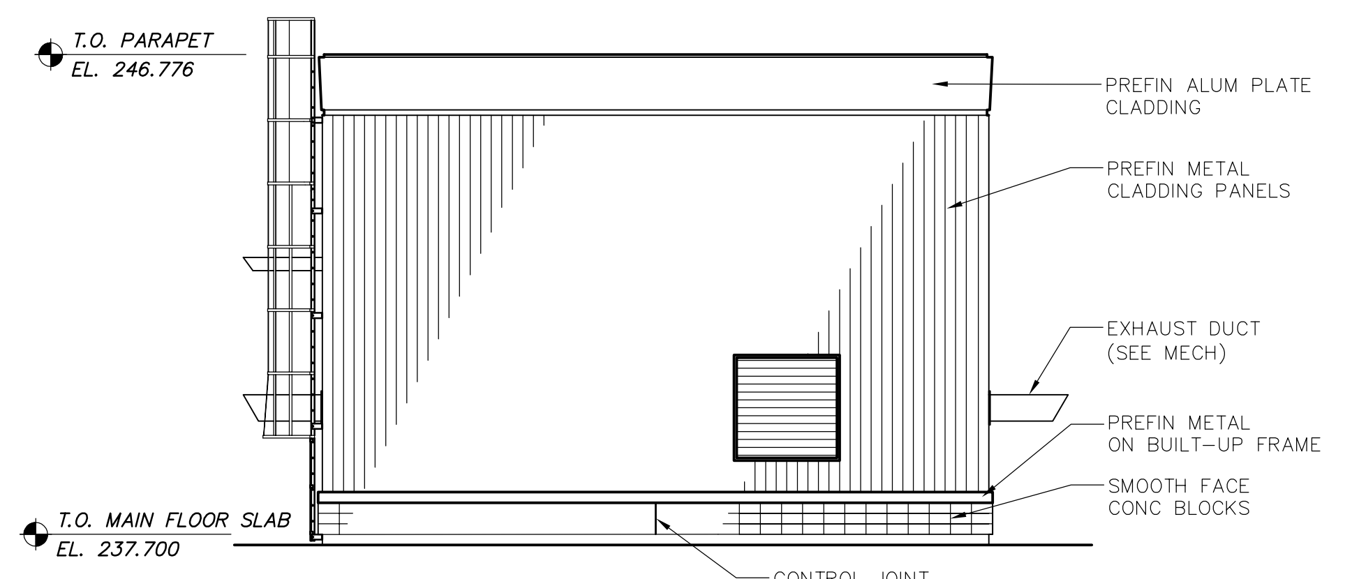
4 WEST ELEVATION WG-B0301 1:100
