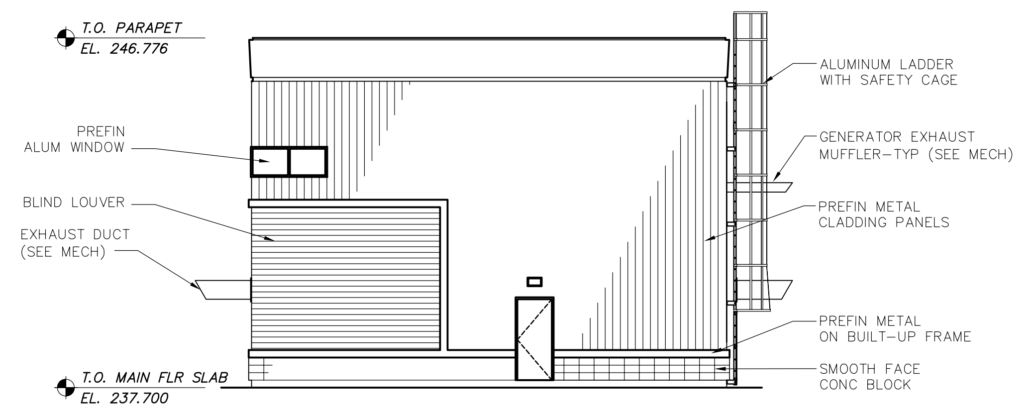
3 EAST ELEVATION WG-B0301 1:100
