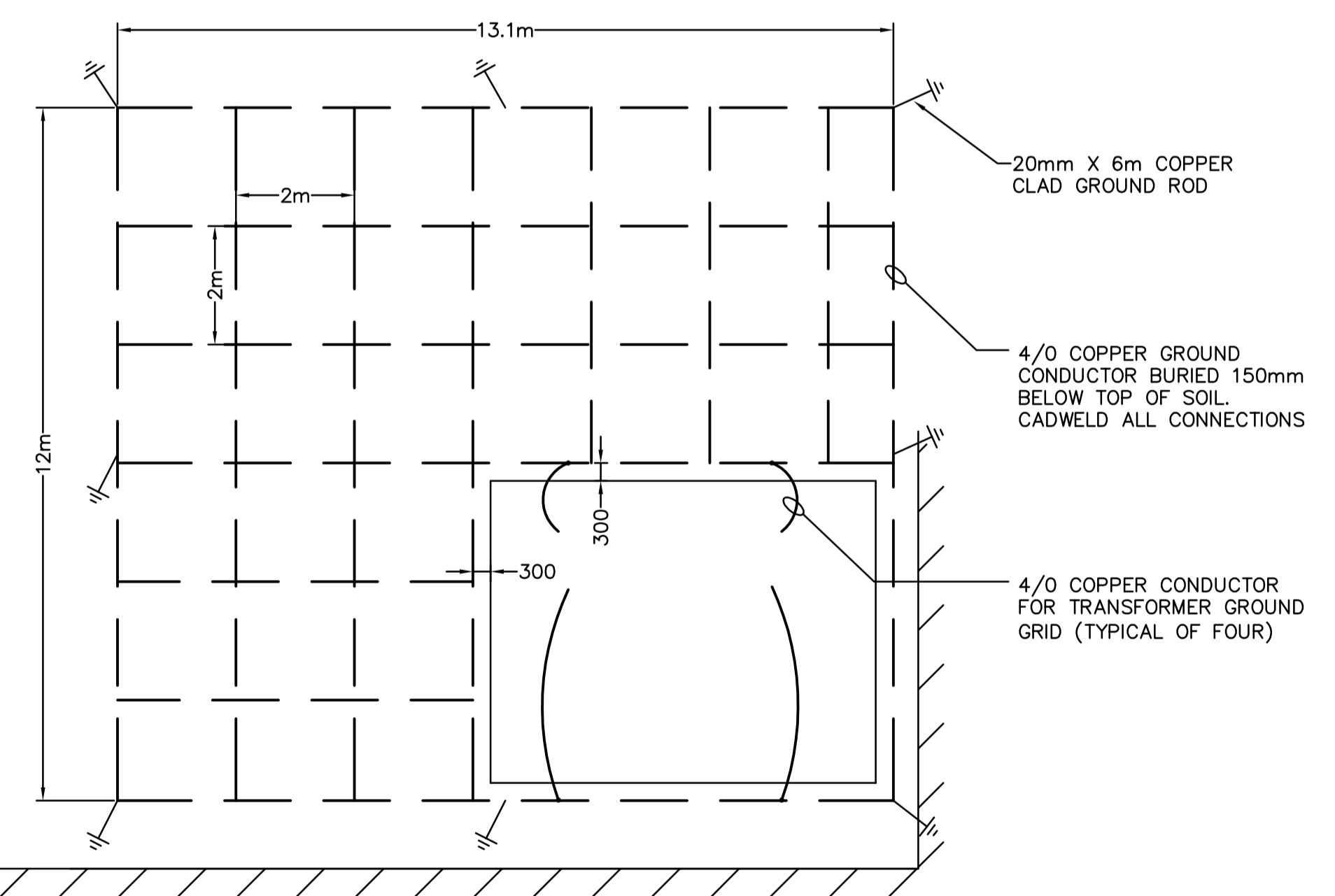
B DETAIL - WTP 4160/600V TRANSFORMER GROUND GRID WG-E0001 NTS
