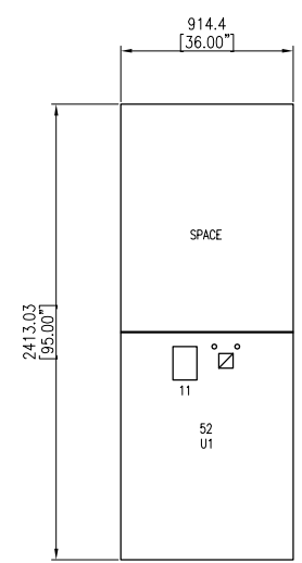
UV BREAKER
