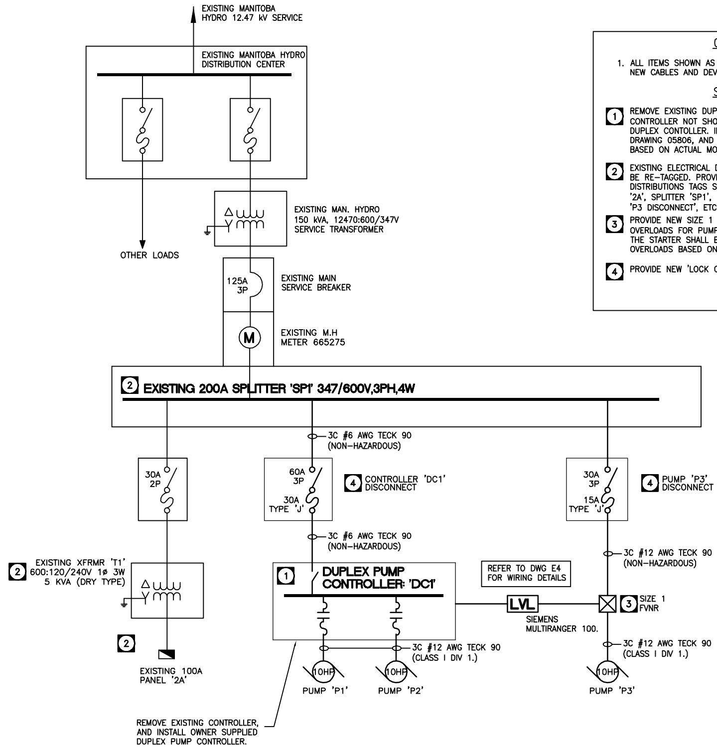
ELECTRICAL SINGLE LINE SCALE: NTS
